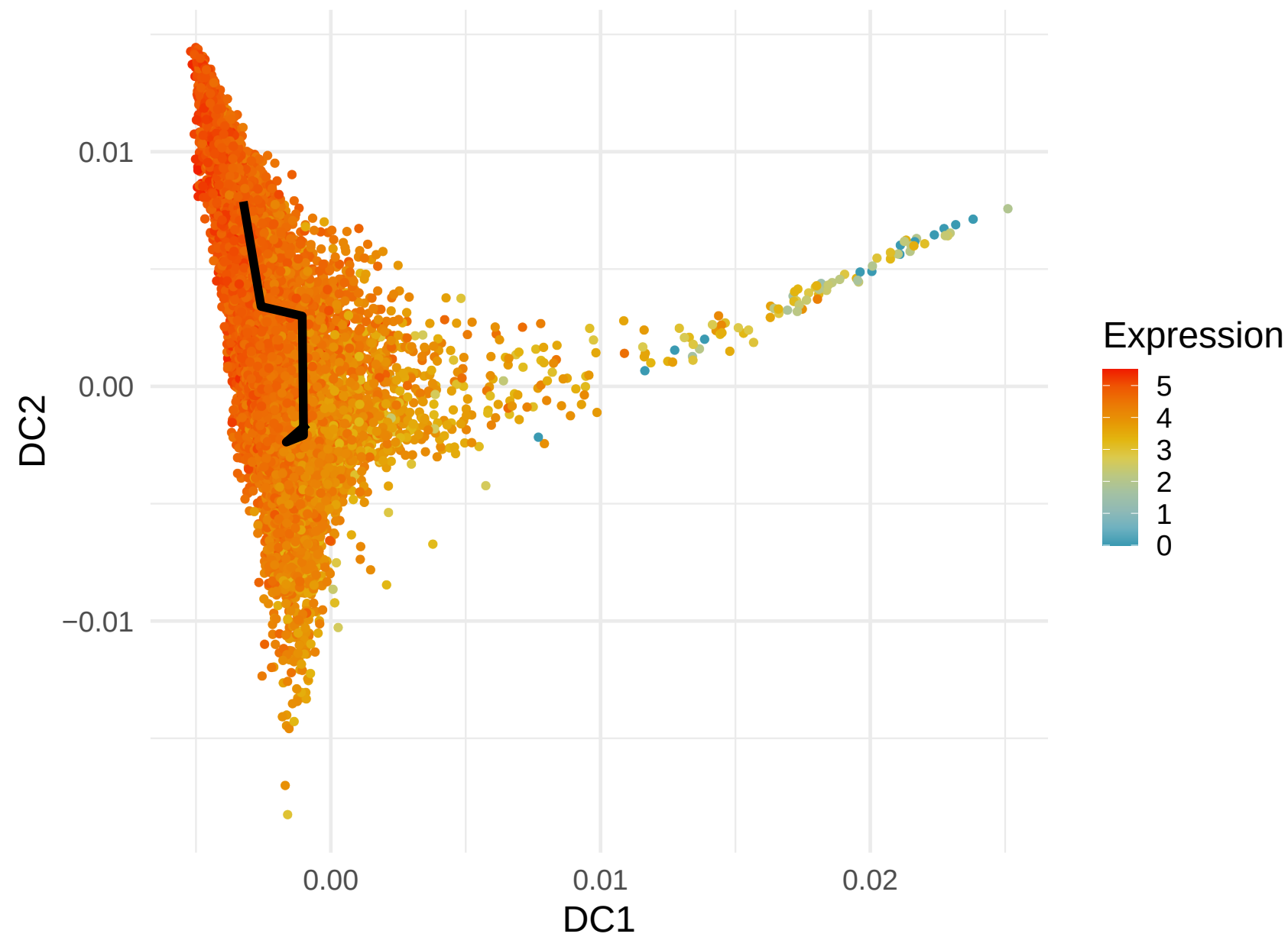
RPS12 Expression along Lineage 1 ( R = -0.324 )
