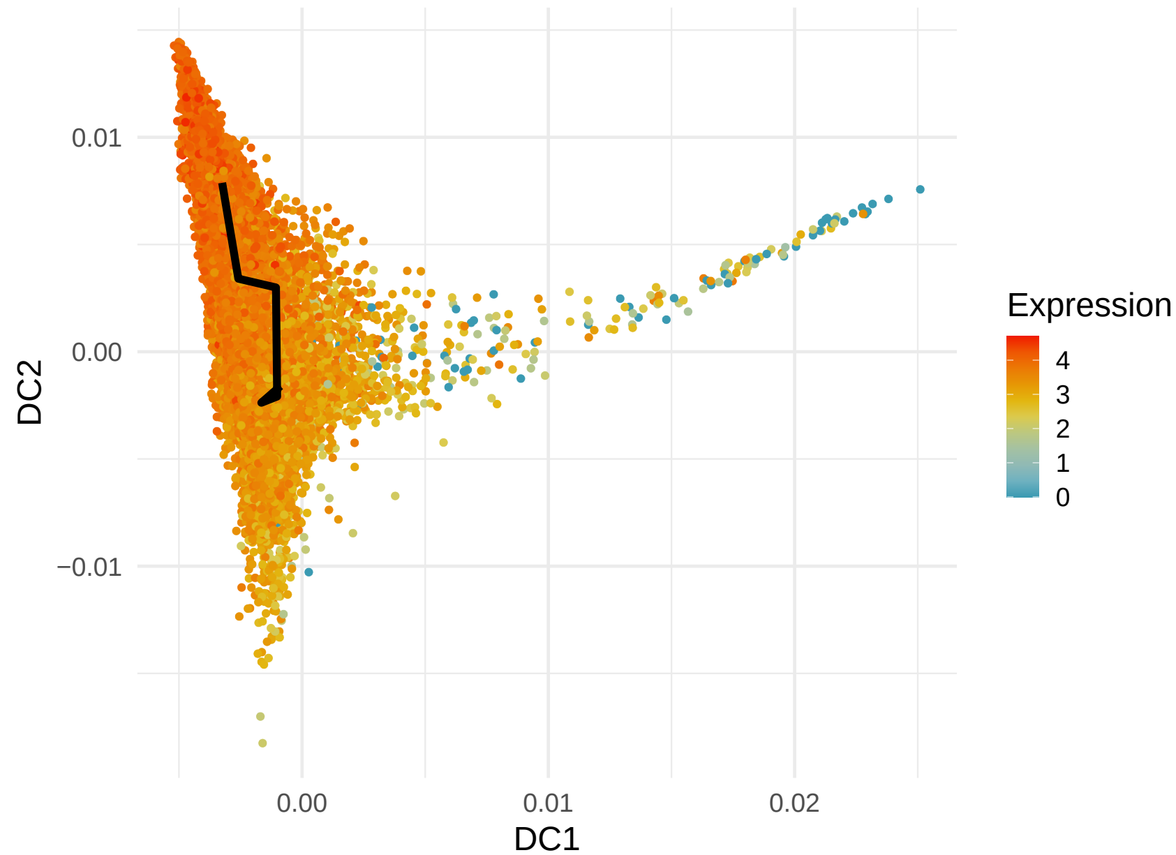
RPS13 Expression along Lineage 1 ( R = -0.299 )
