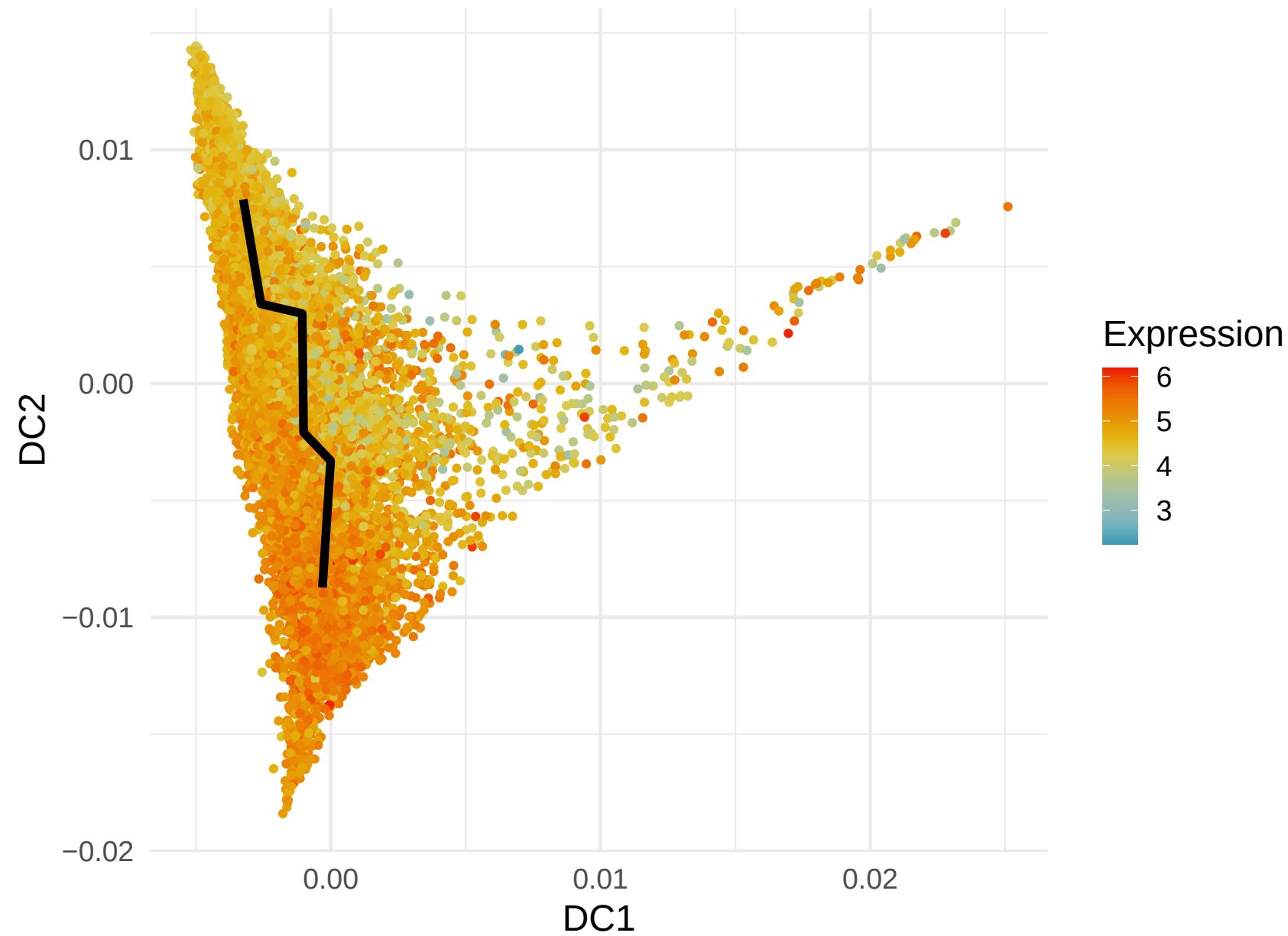
B2M Expression along Lineage 2 ( R = 0.472 )
