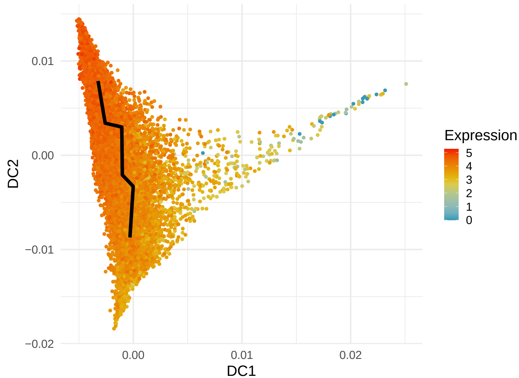
RPL30 Expression along Lineage 2 ( R = -0.444 )
