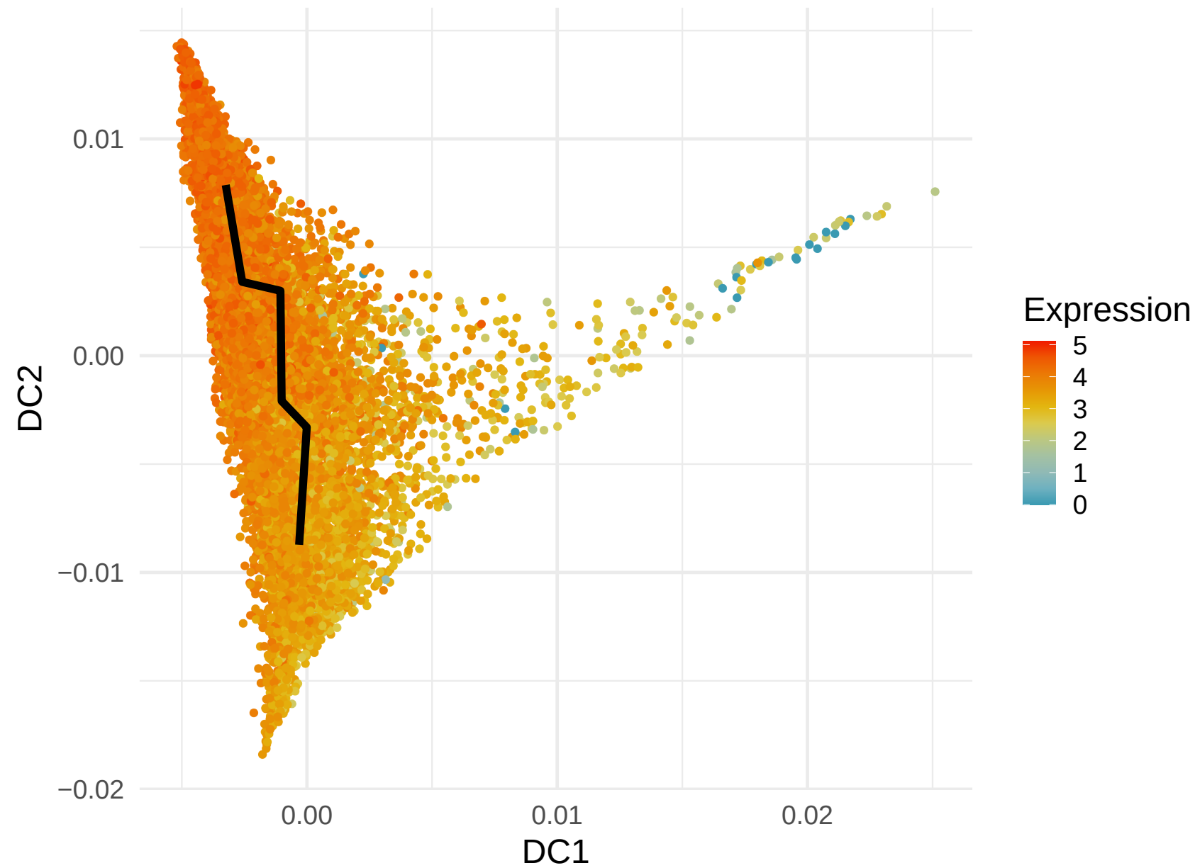
RPS8 Expression along Lineage 2 ( R = -0.441 )
