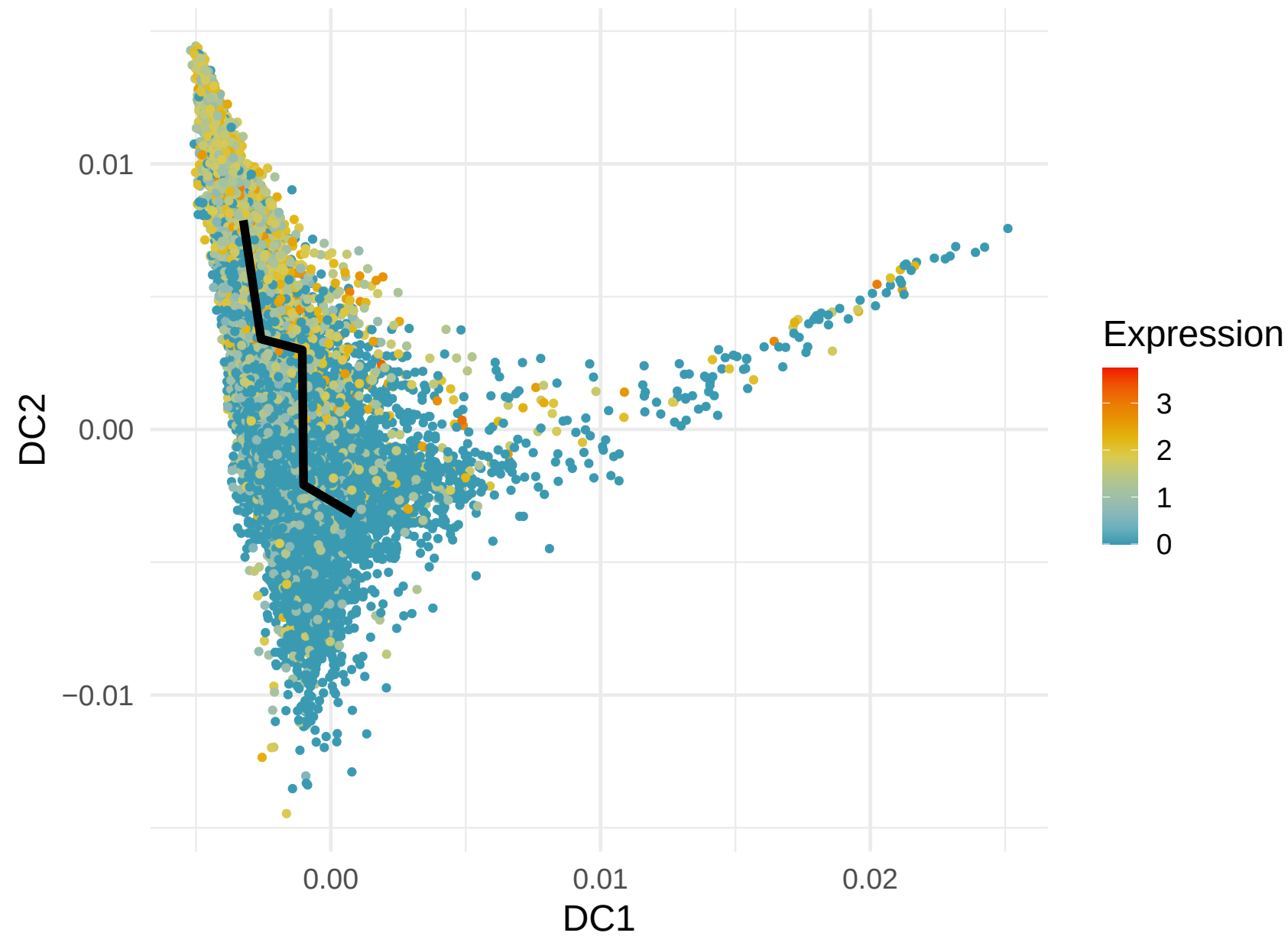
CCR7 Expression along Lineage 3 ( R = -0.477 )
