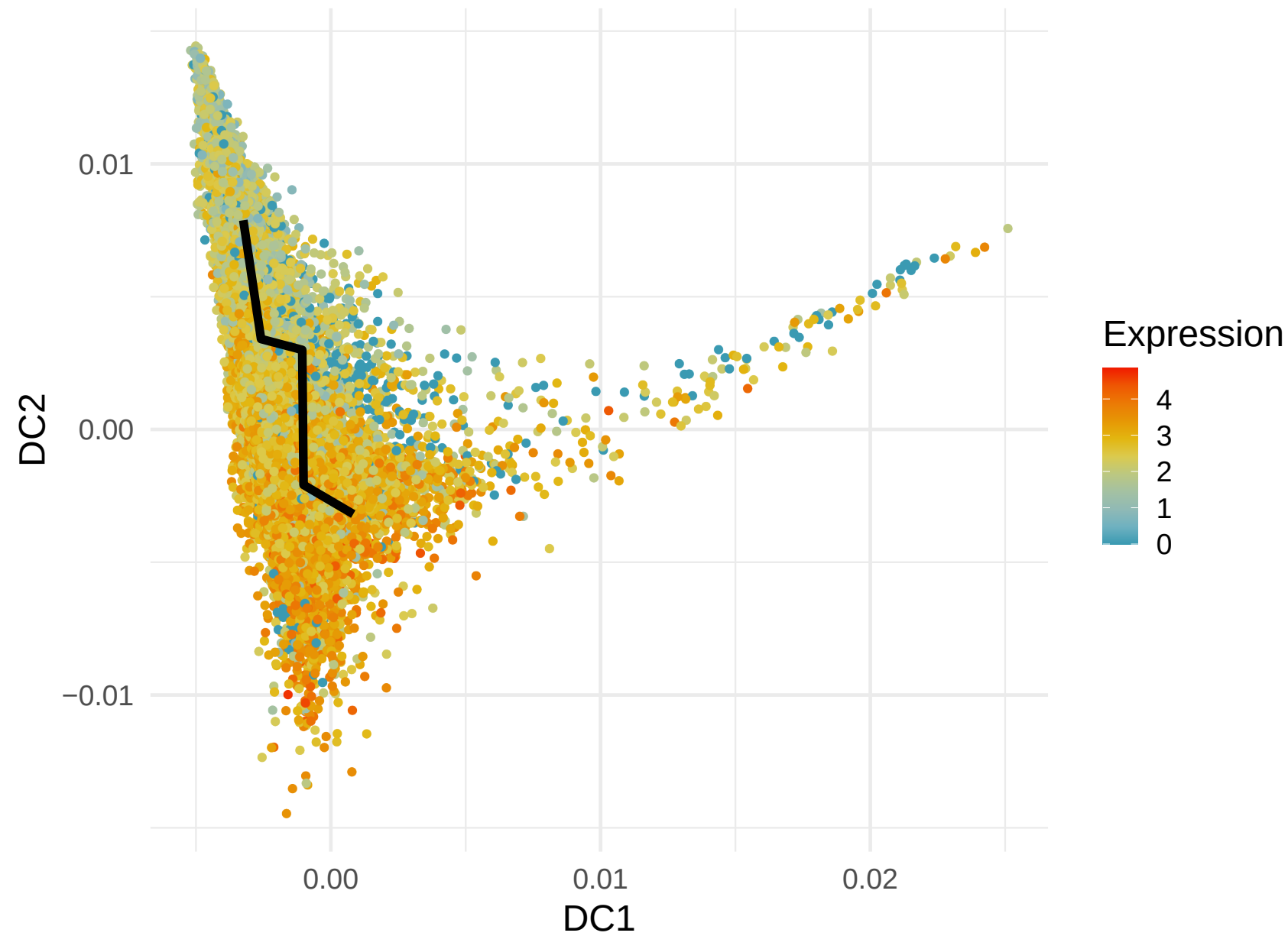
IL32 Expression along Lineage 3 ( R = 0.369 )
