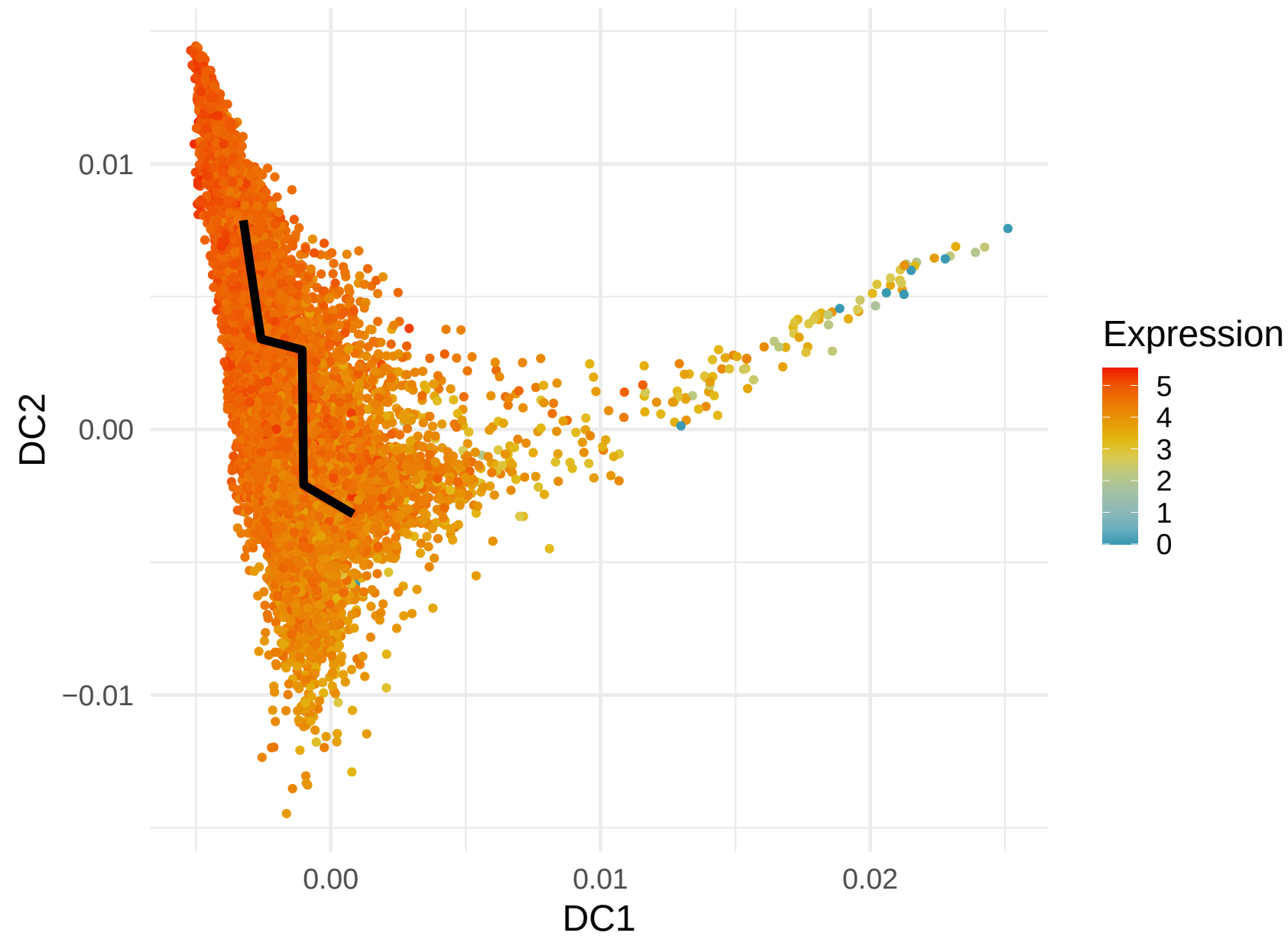
RPL13 Expression along Lineage 3 ( R = -0.495 )
