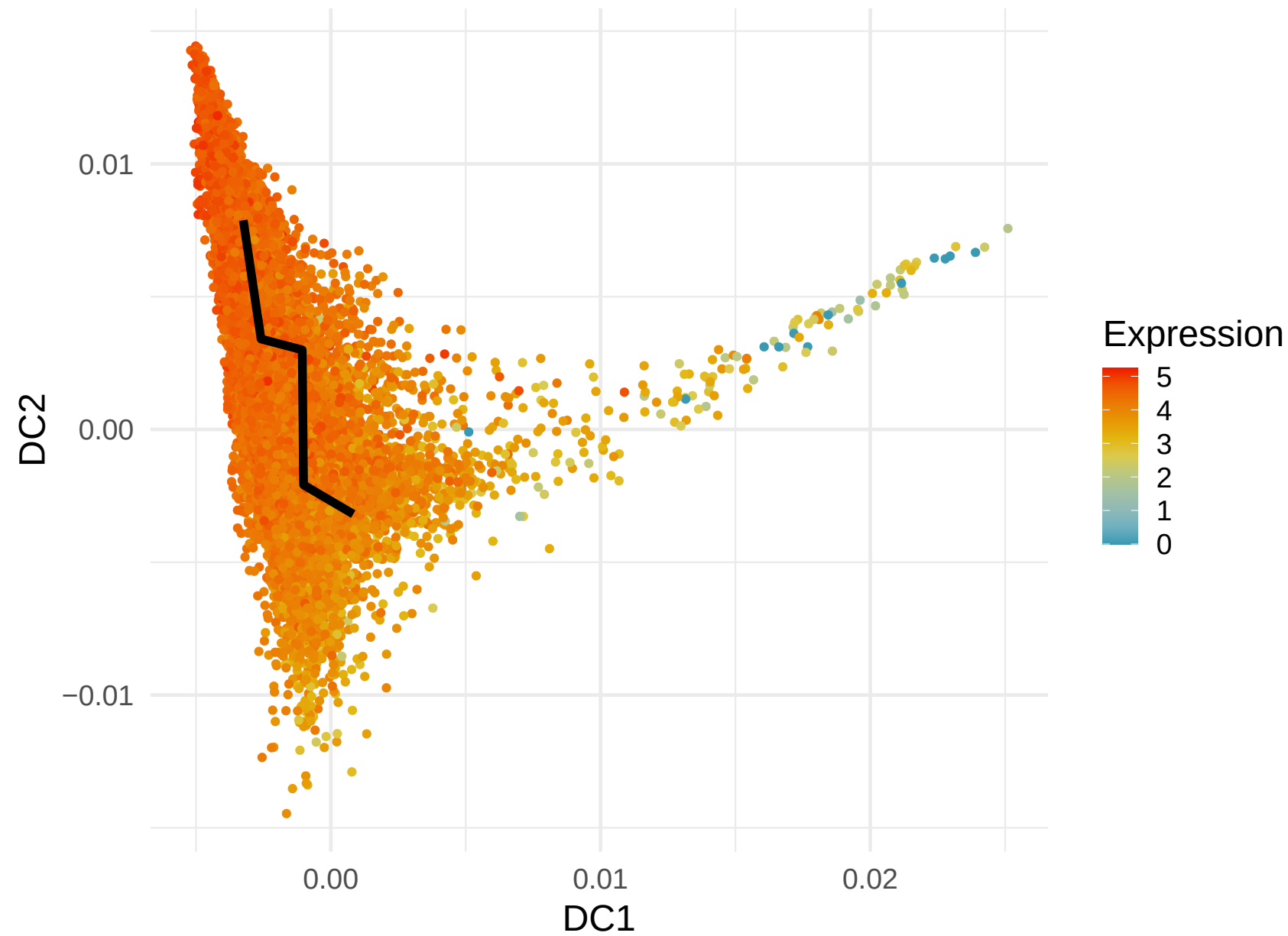
RPL32 Expression along Lineage 3 ( R = -0.497 )
