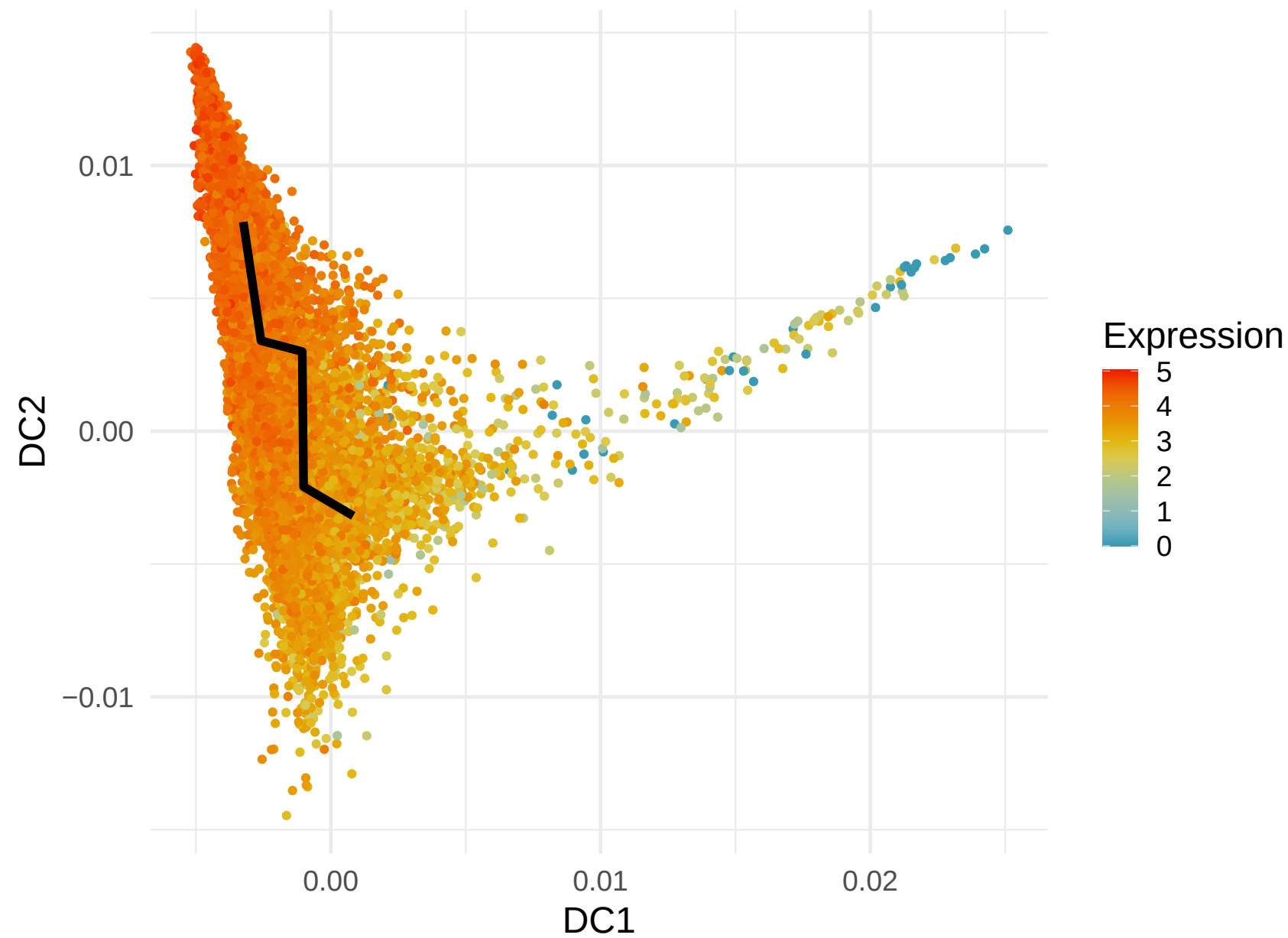
RPS3A Expression along Lineage 3 ( R = -0.514 )
