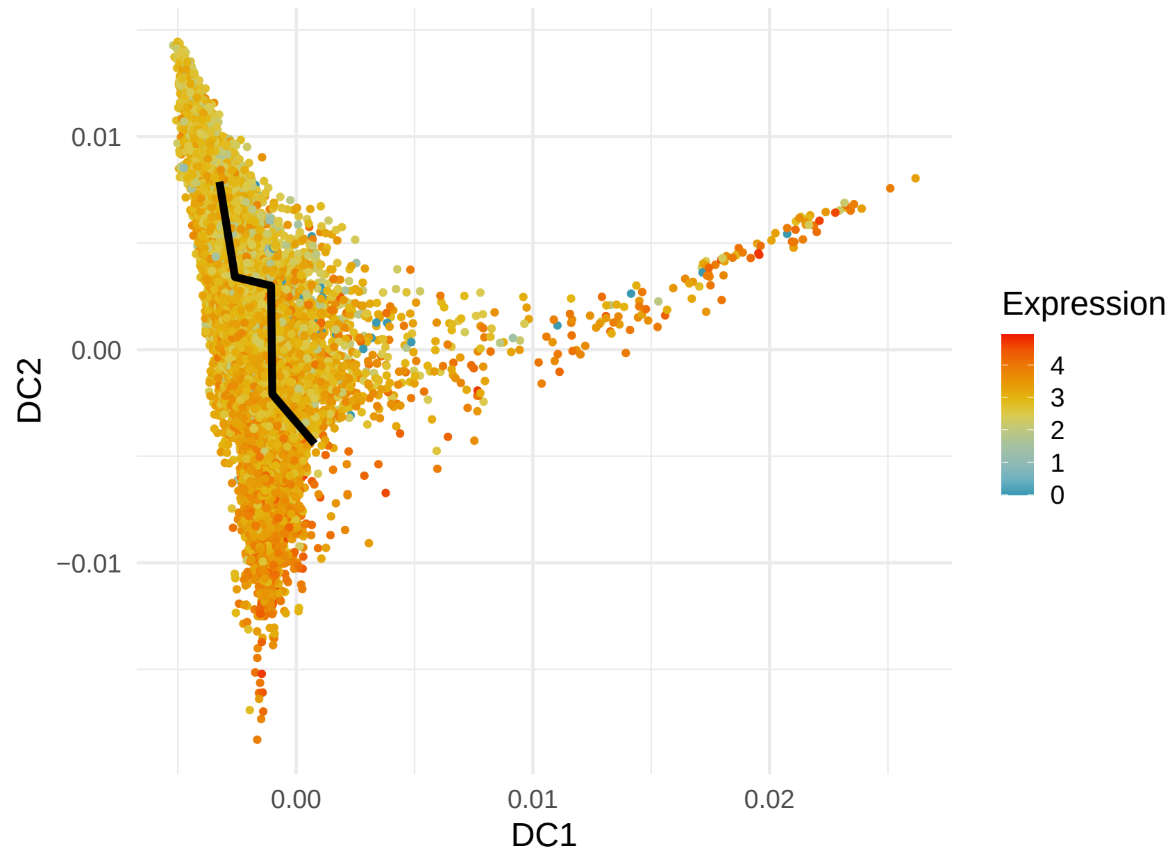
HLA-A Expression along Lineage 4 ( R = 0.367 )
