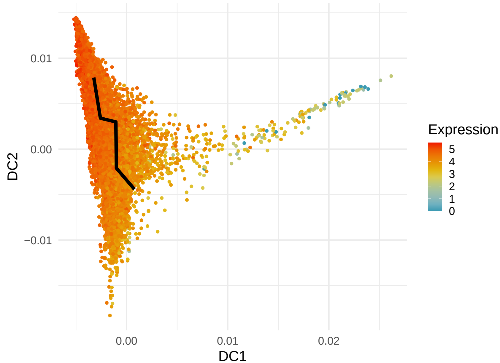
RPS12 Expression along Lineage 4 ( R = -0.48 )
