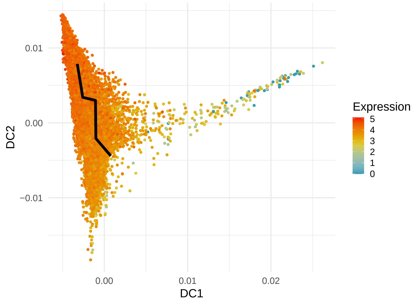
RPS23 Expression along Lineage 4 ( R = -0.442 )
