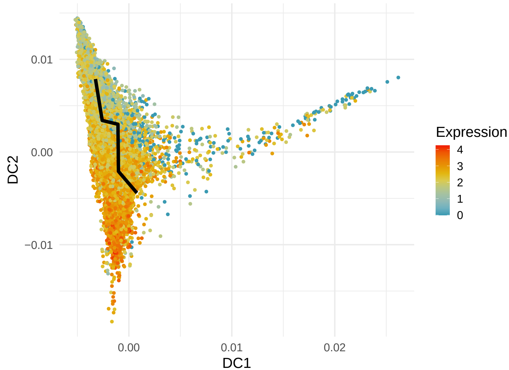
SH3BGRL3 Expression along Lineage 4 ( R = 0.439 )
