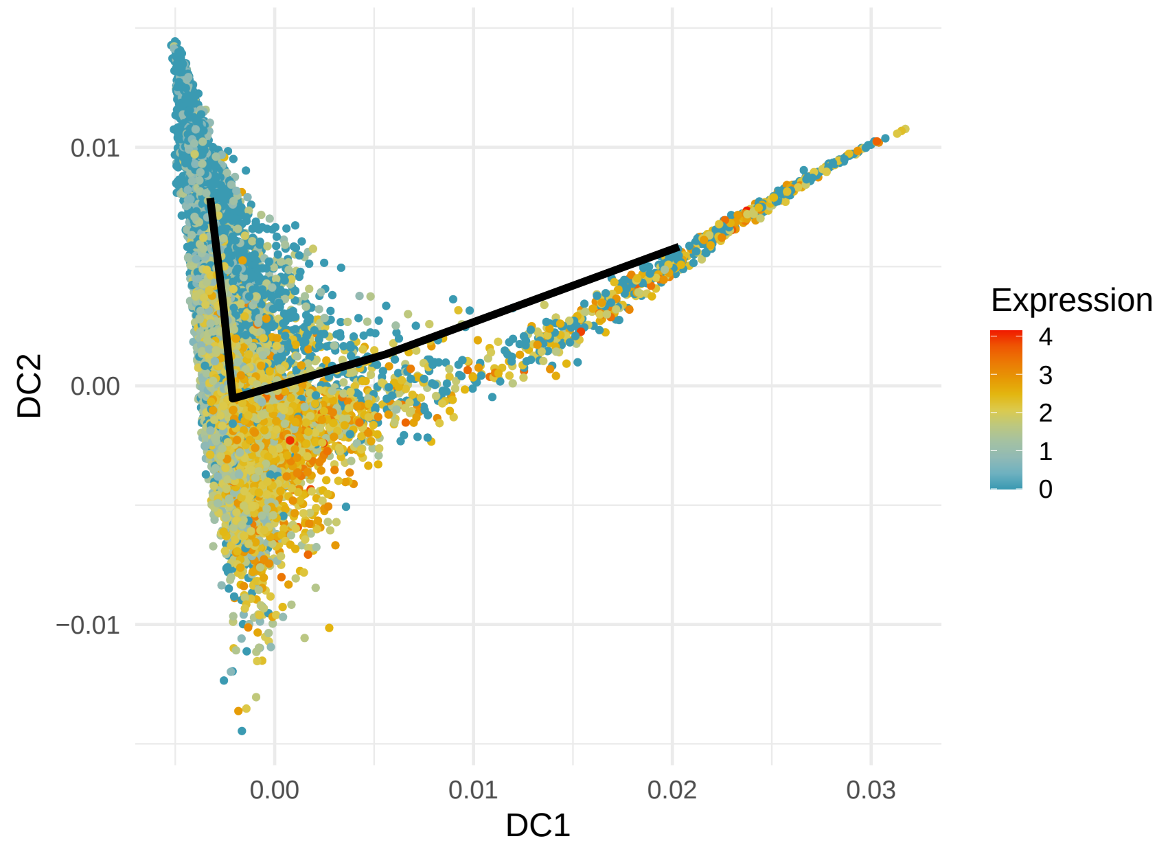
AHNAK Expression along Lineage 5 (R= 0.382)
