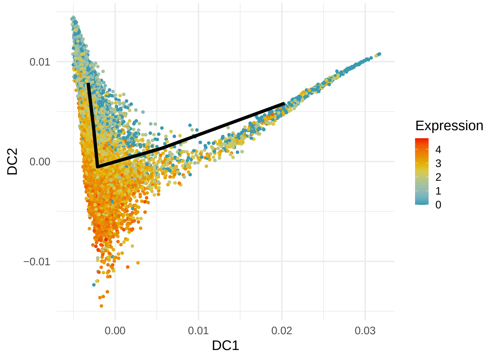
S100A4 Expression along Lineage 5 ( R = 0.313 )
