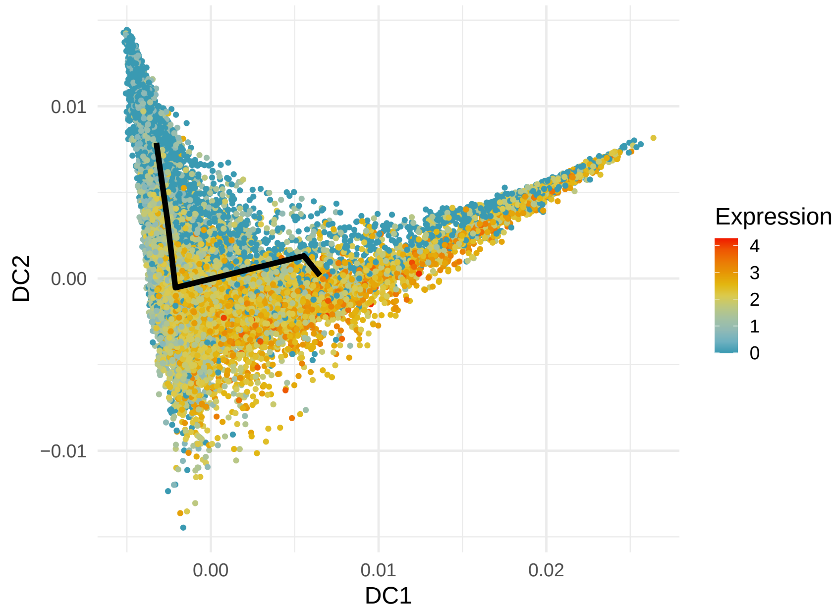
AHNAK Expression along Lineage 6 ( R = 0.5 )
