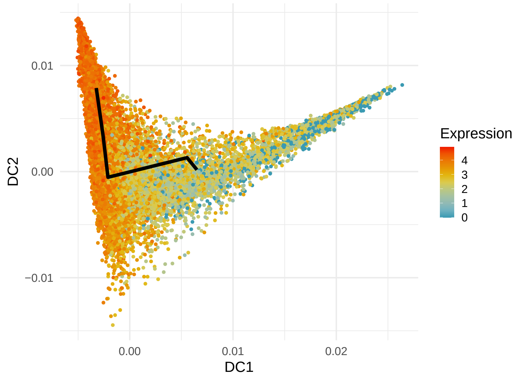
RPL21 Expression along Lineage 6 ( R = -0.601 )
