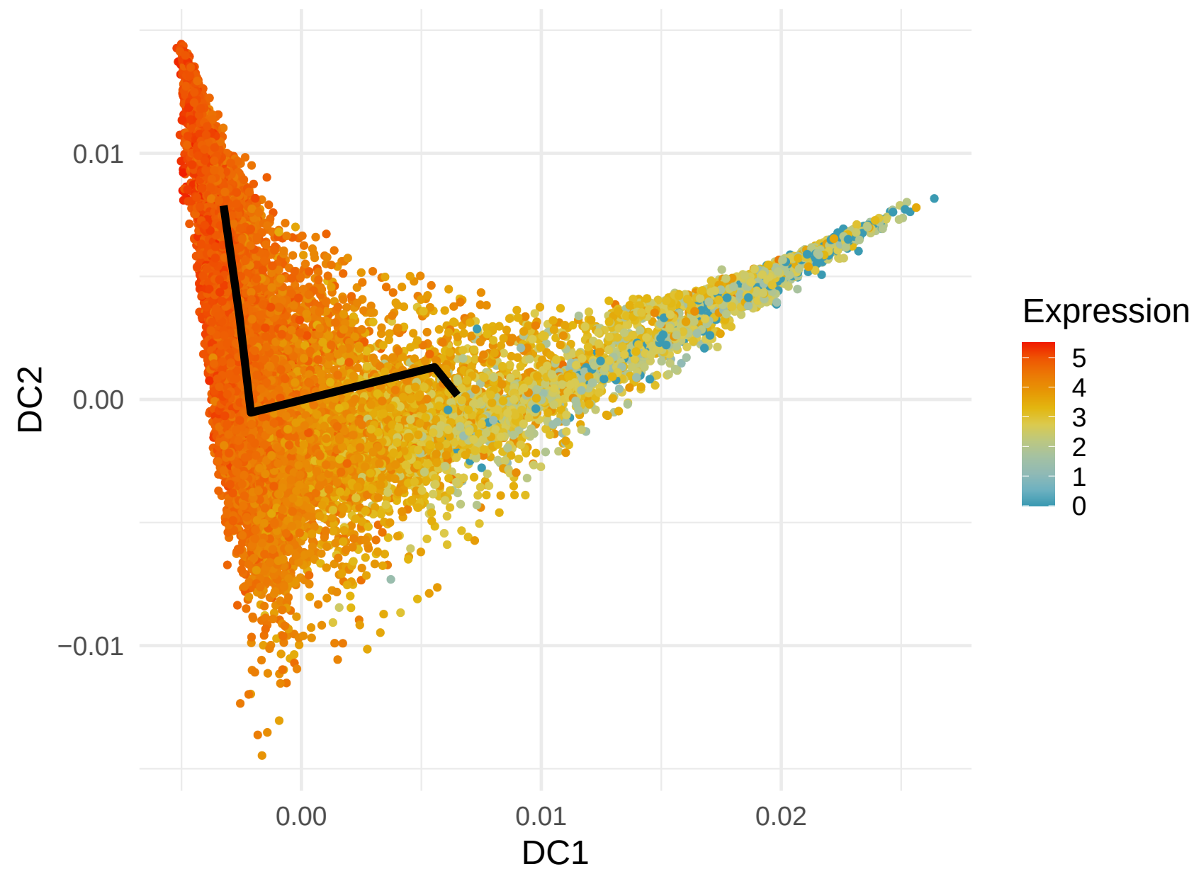
RPS12 Expression along Lineage 6 ( R = -0.596 )
