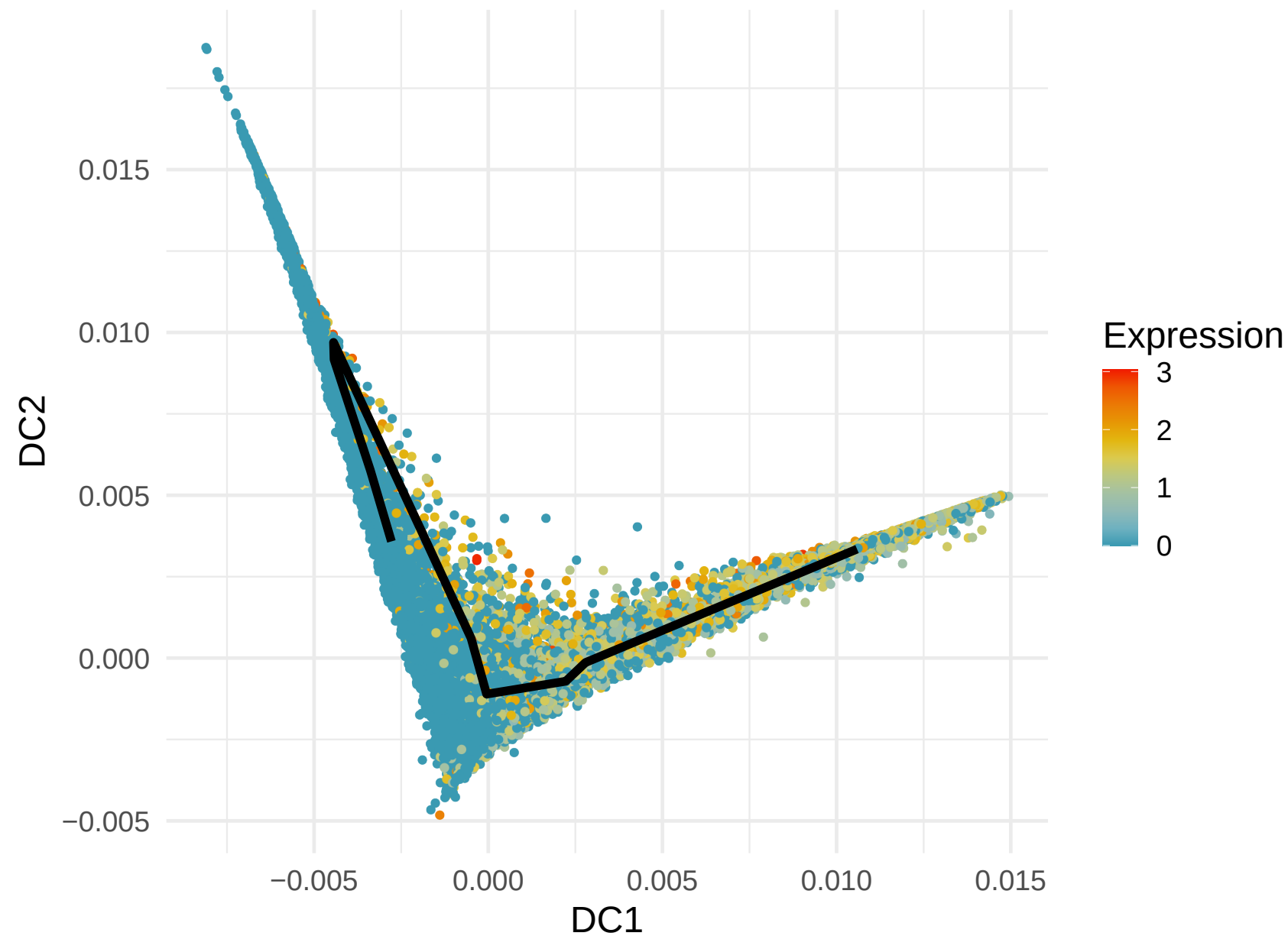
RCAN3 Expression along Lineage 1 ( R = -0.543 )
