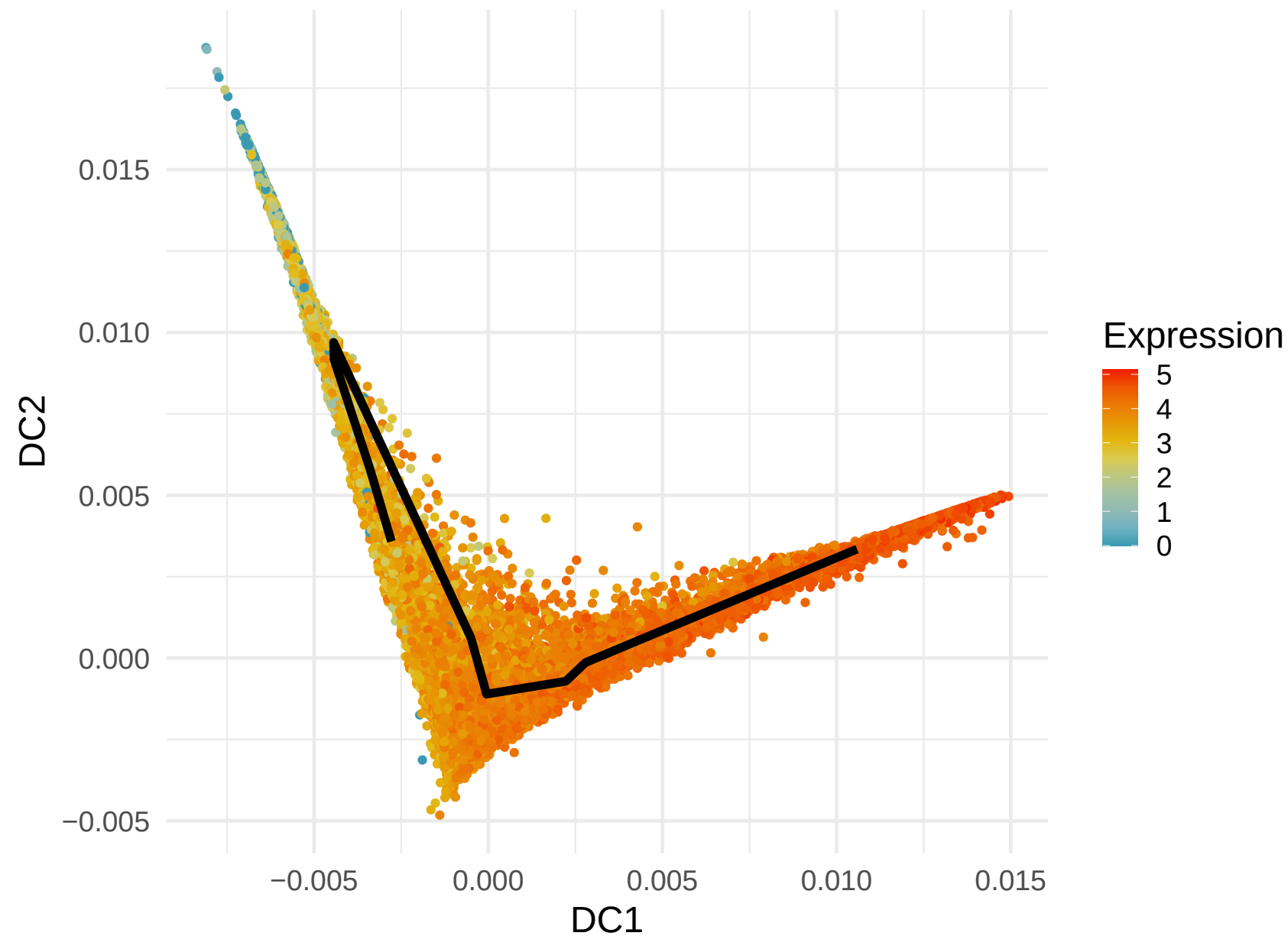
RPL32 Expression along Lineage 1 ( R = -0.521 )
