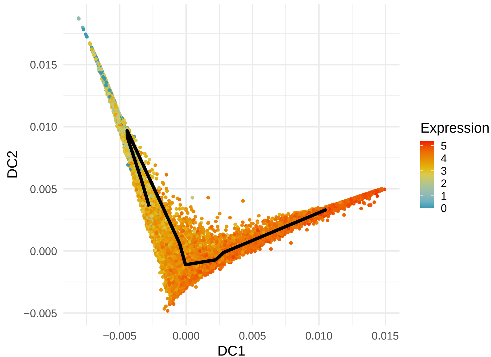
RPLP1 Expression along Lineage 1 ( R = -0.547 )
