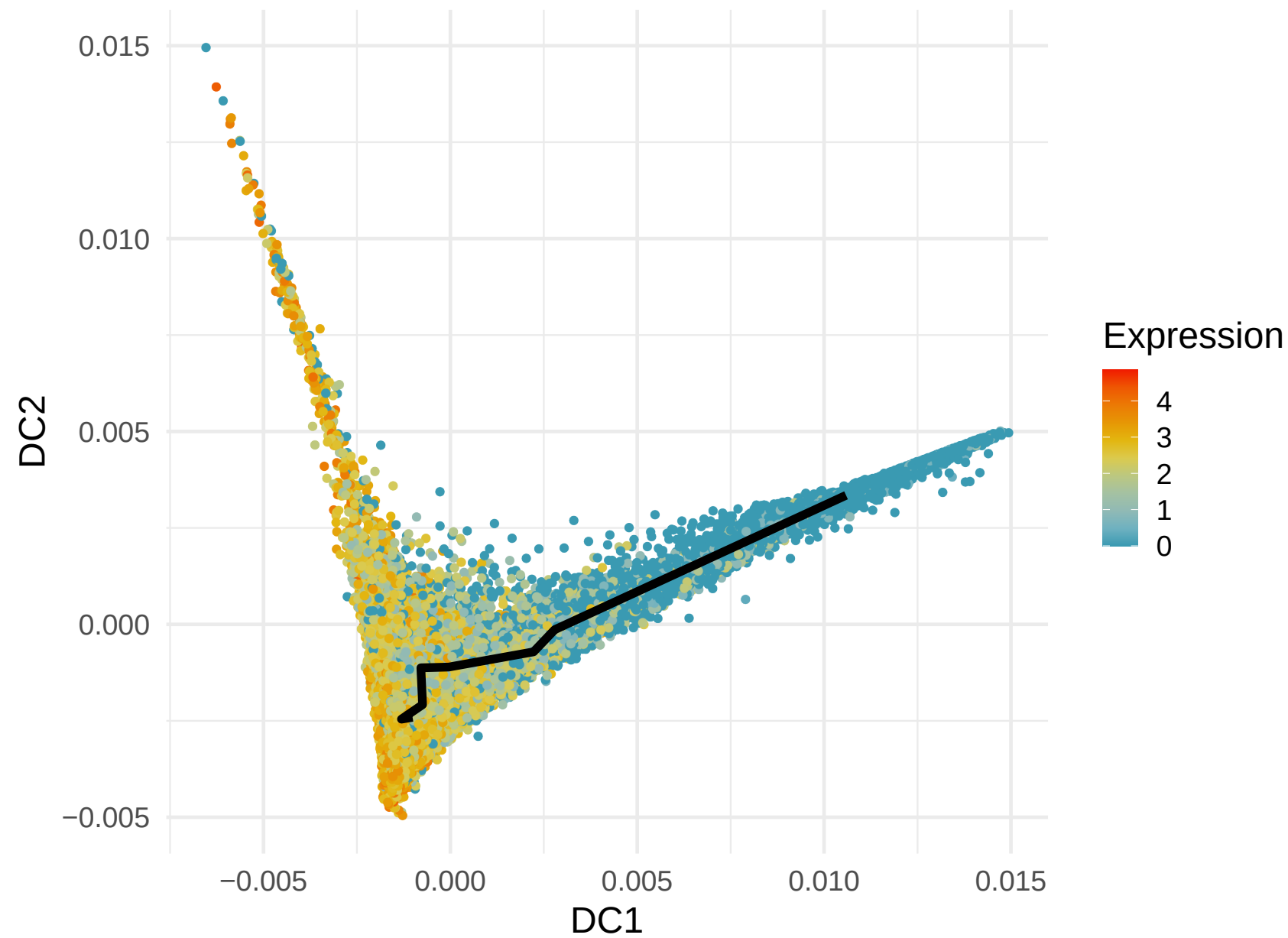
GZMA Expression along Lineage 2 ( R = 0.649 )
