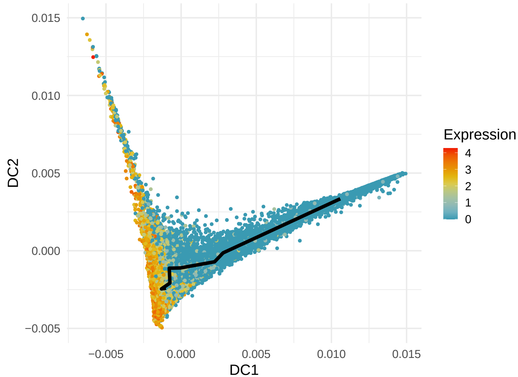
GZMH Expression along Lineage 2 (R= 0.715)
