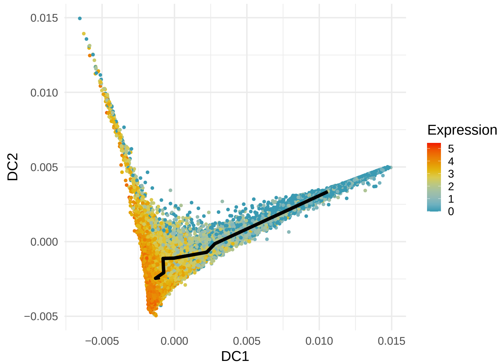
NKG7 Expression along Lineage 2 ( R = 0.835 )
