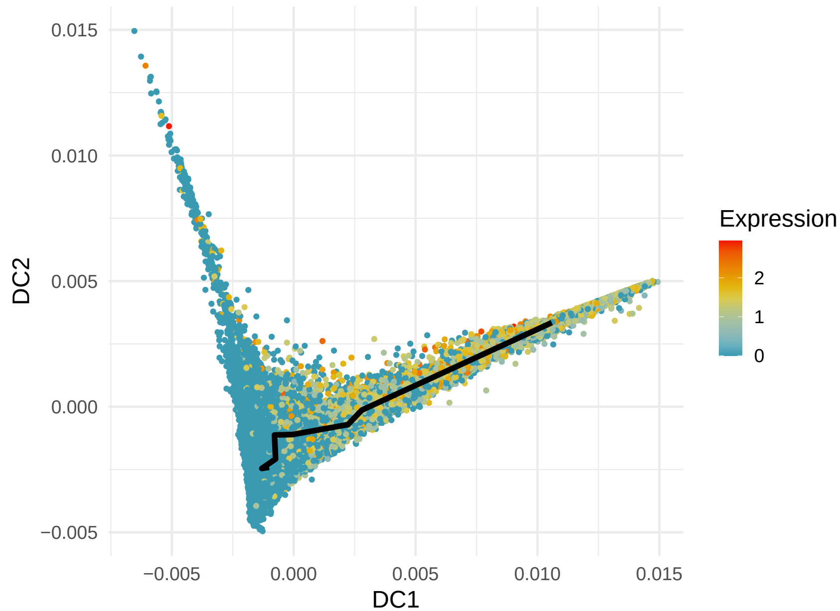
RCAN3 Expression along Lineage 2 ( R = -0.612 )
