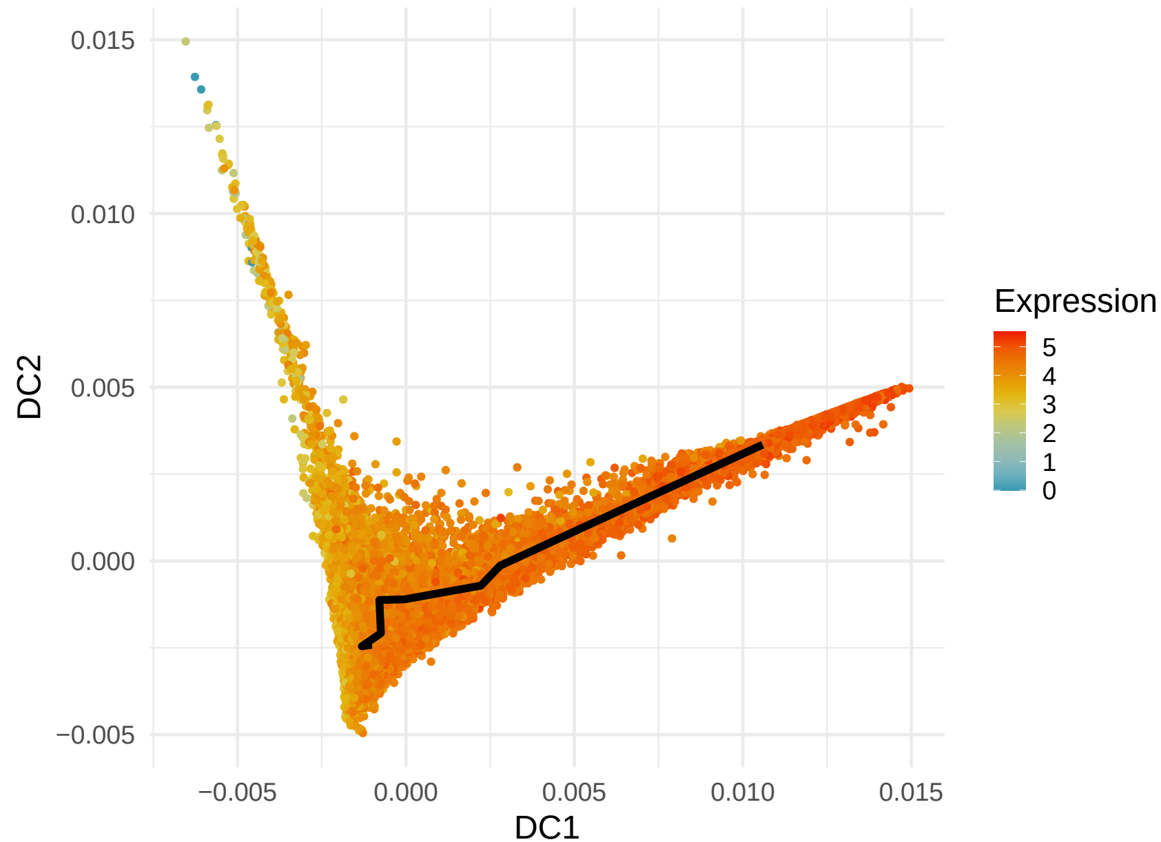
RPL13 Expression along Lineage 2 ( R = -0.593 )
