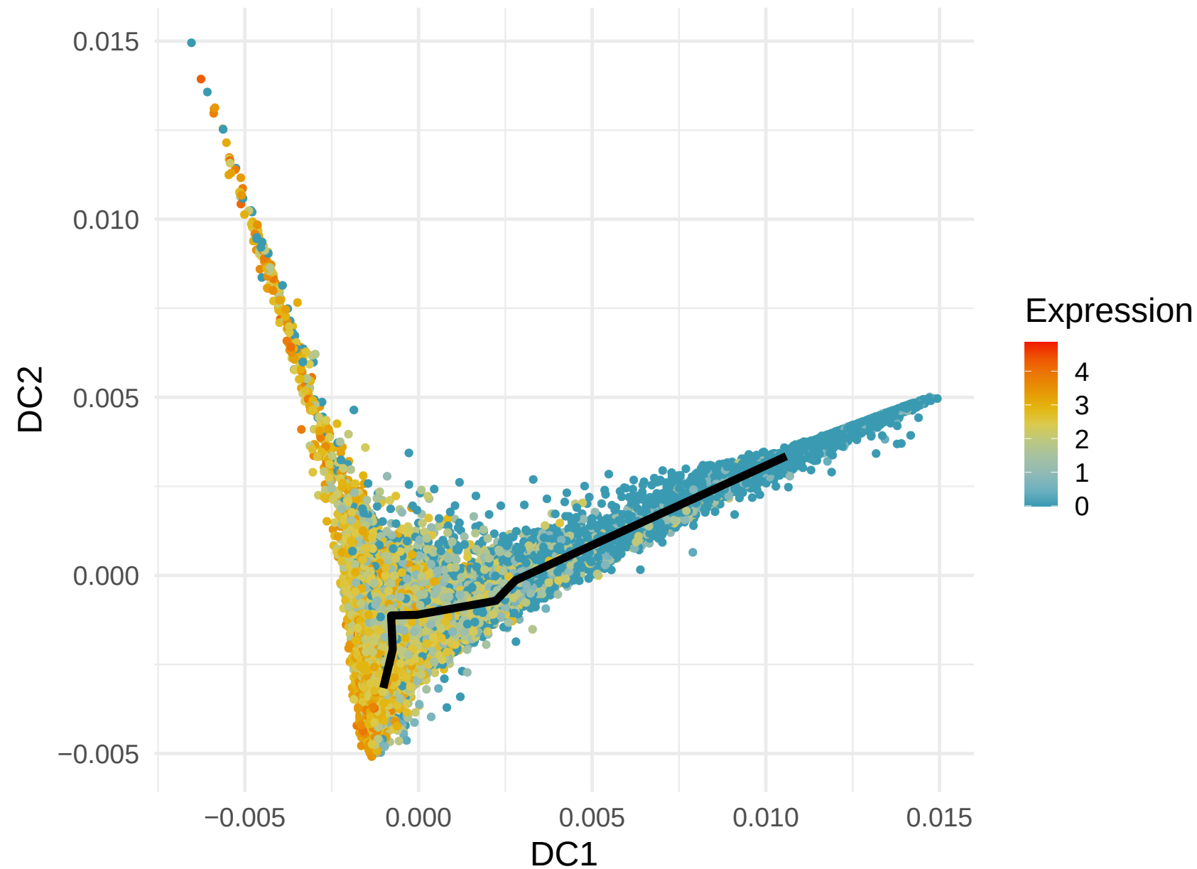
GZMA Expression along Lineage 3 ( R = 0.64 )
