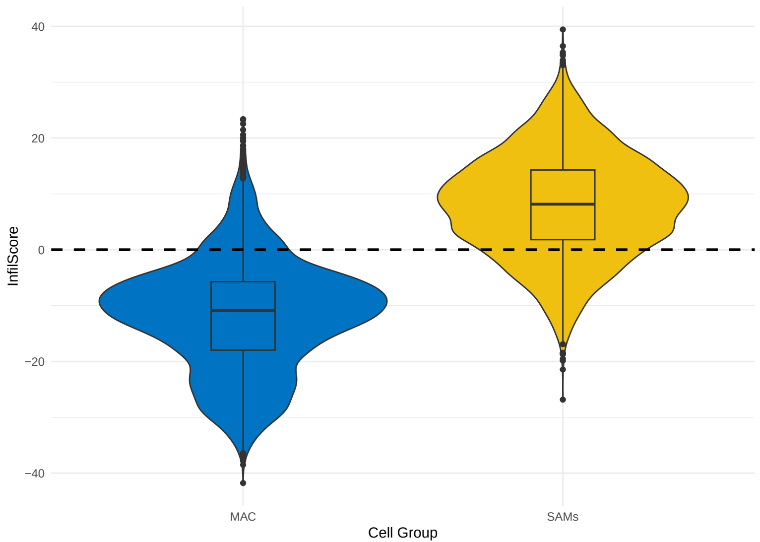
SAM Scores in Macrophage Subtypes
