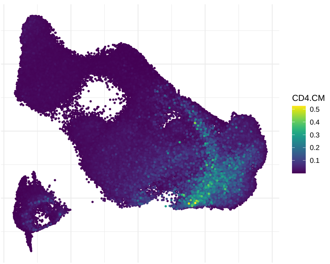
TCAT CD4 Central Memory Usage
