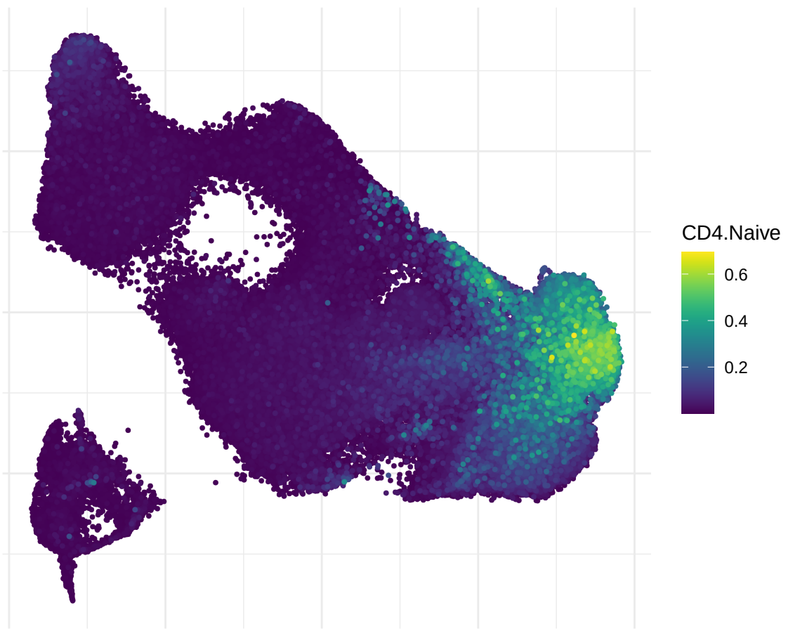
TCAT CD4 Naive Usage
