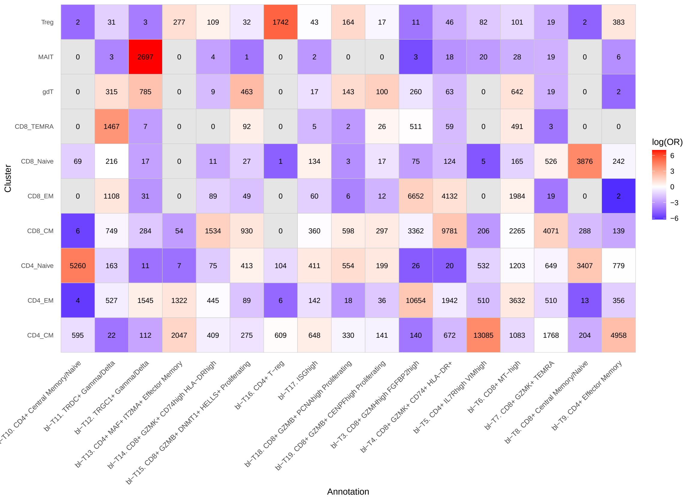
T Cluster Enrichment Heatmap
