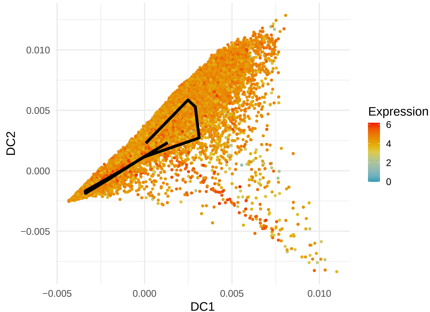
MT-CO2 Expression along Lineage 1 ( R = -0.221 )
