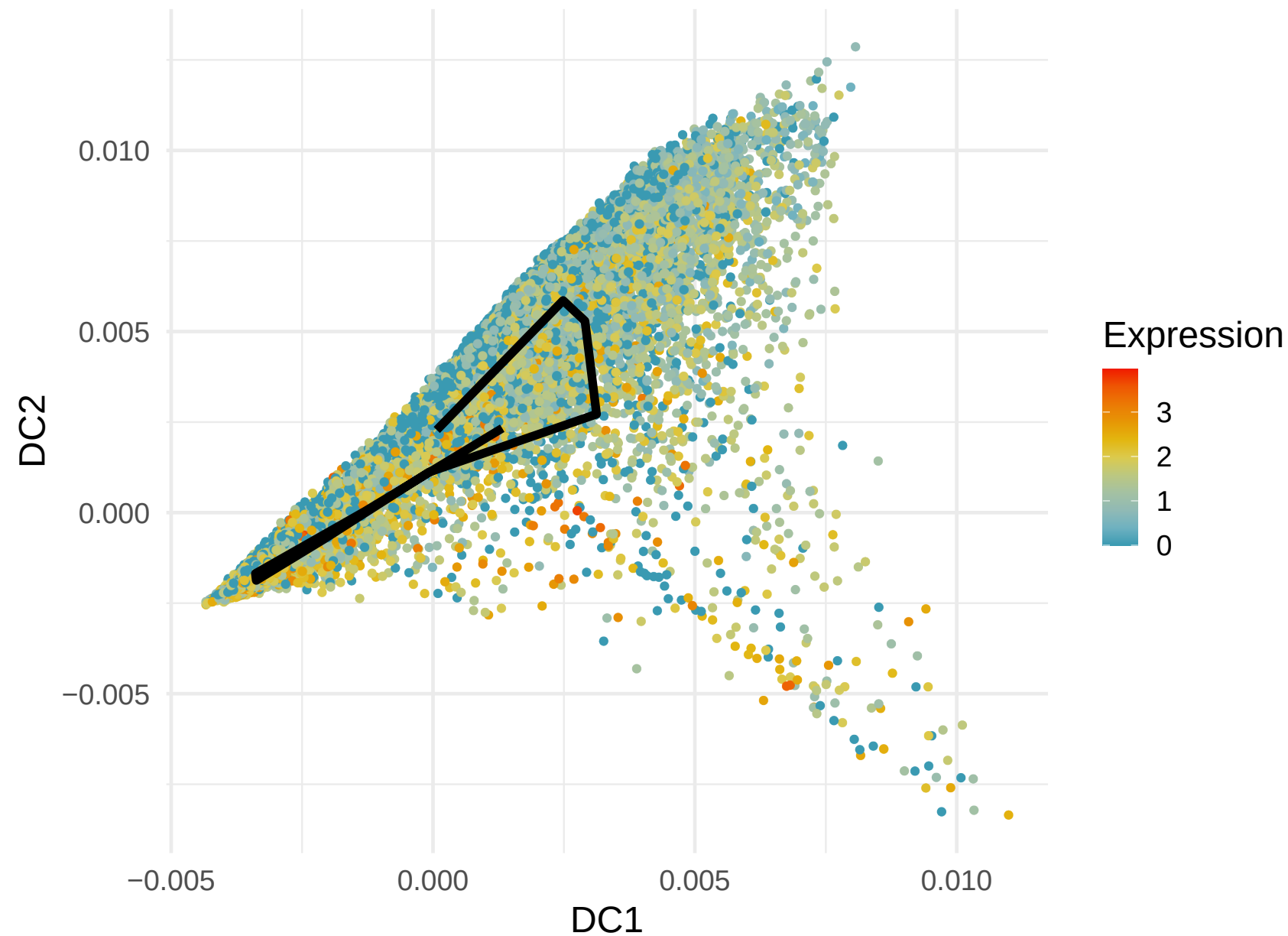
STX7 Expression along Lineage 1 ( R = -0.21 )
