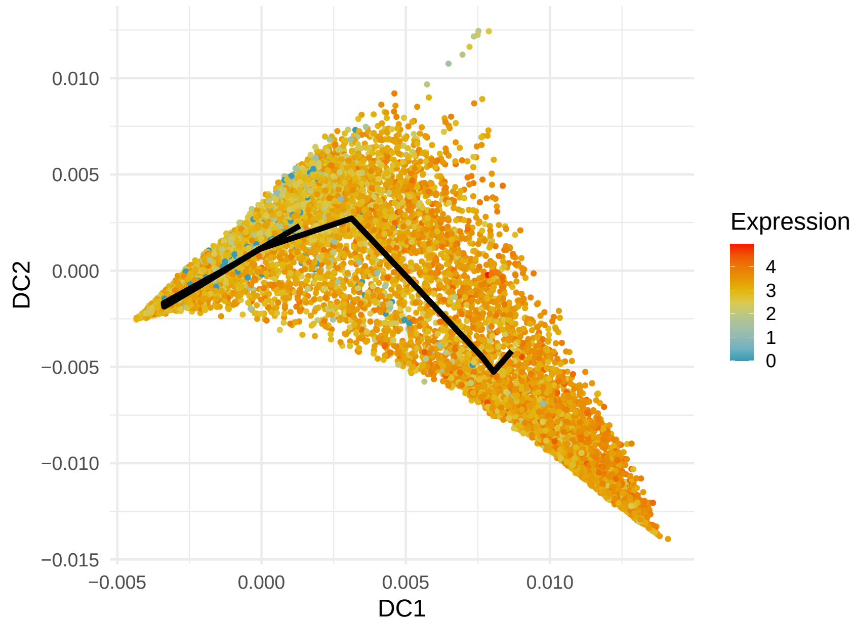
CD52 Expression along Lineage 2 (R= 0.416)
