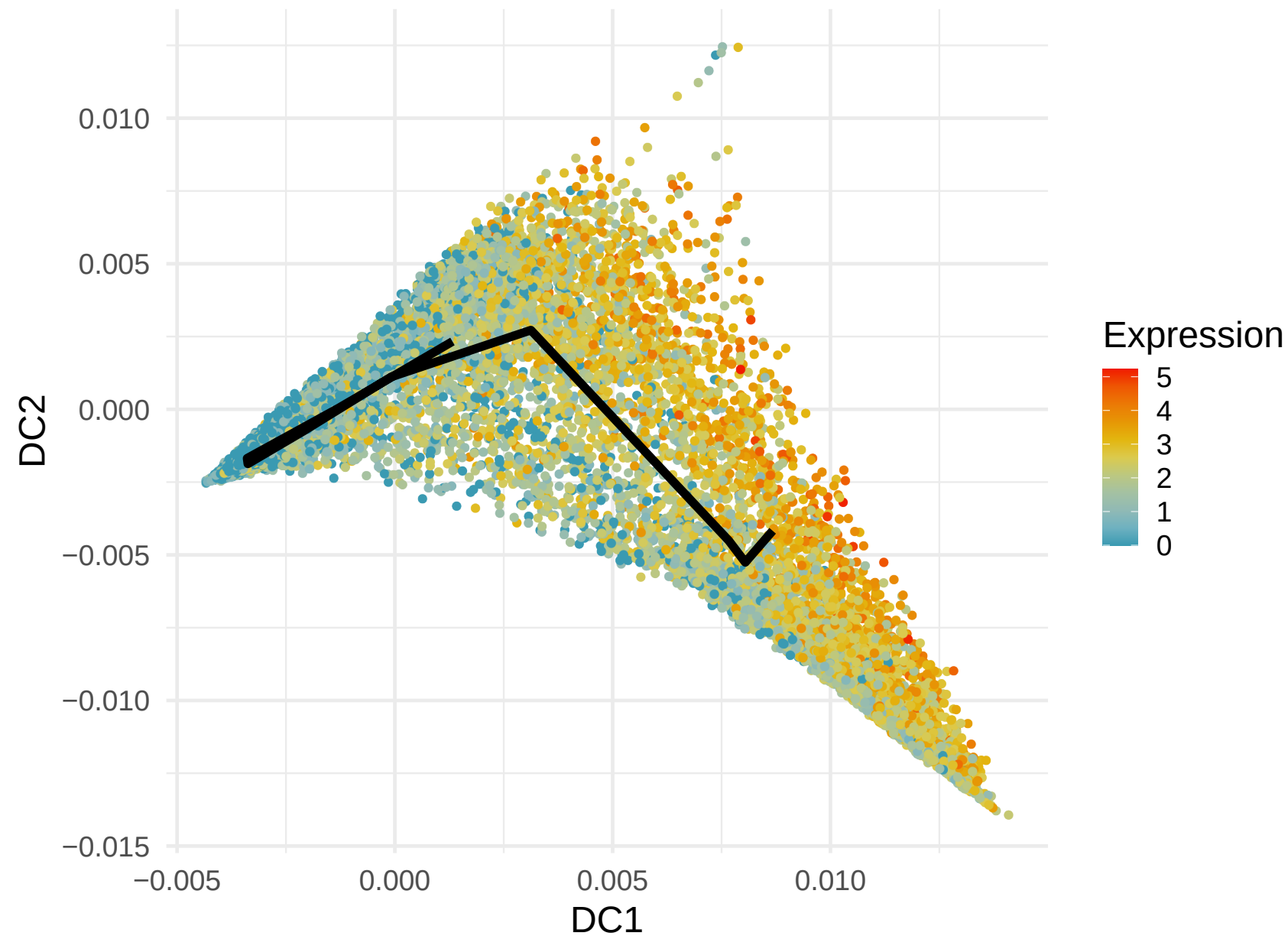
CRIP1 Expression along Lineage 2 (R= 0.393)
