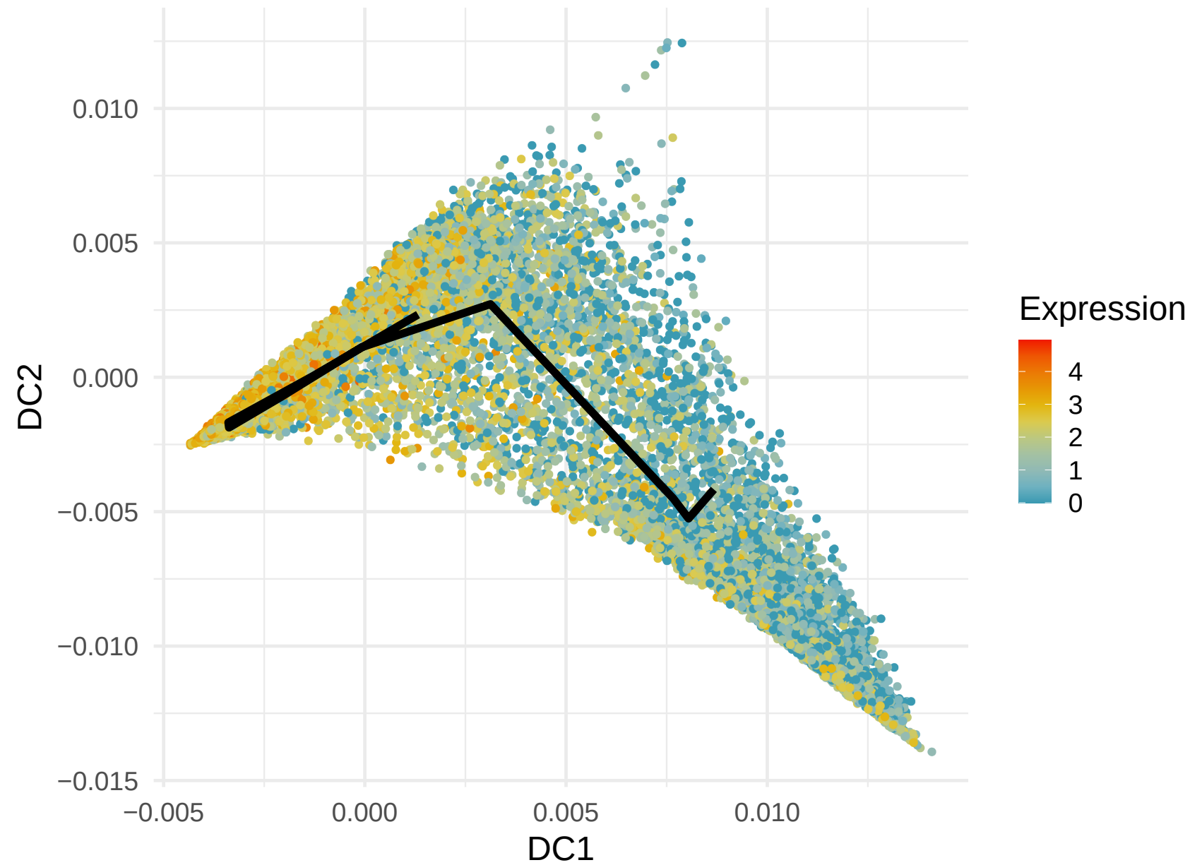
CXCR4 Expression along Lineage 2 ( R = -0.288 )
