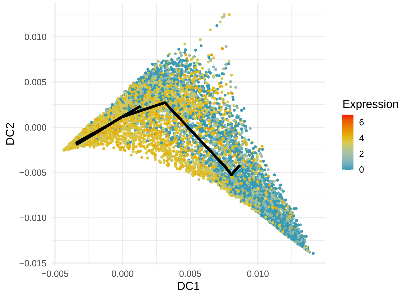
IGHM Expression along Lineage 2 ( R = -0.281 )
