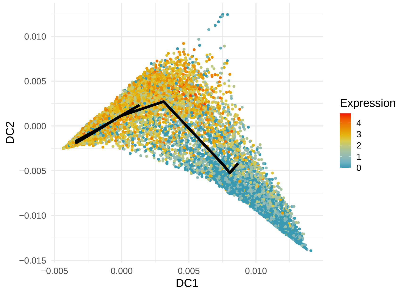
LTB Expression along Lineage 2 ( R = -0.242 )
