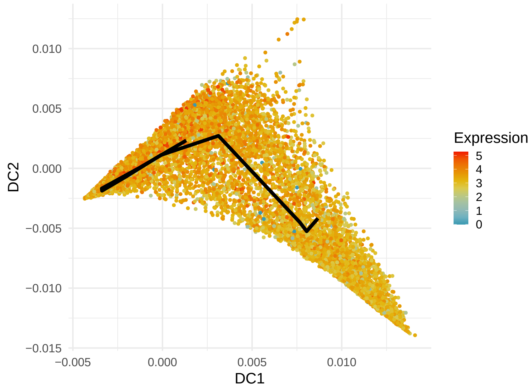
MT-ND1 Expression along Lineage 2 ( R = -0.252 )
