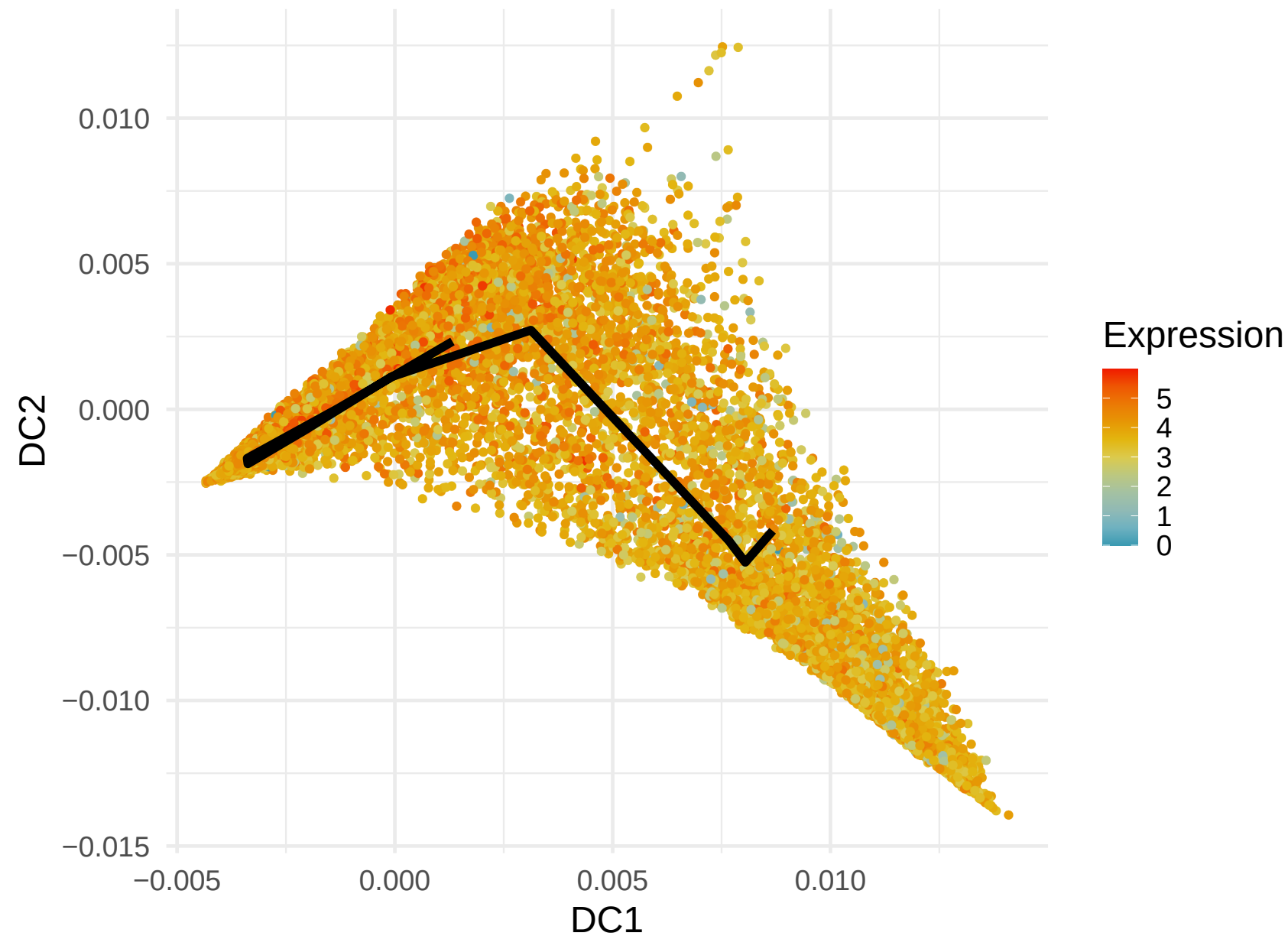
MT-ND3 Expression along Lineage 2 ( R = -0.26 )
