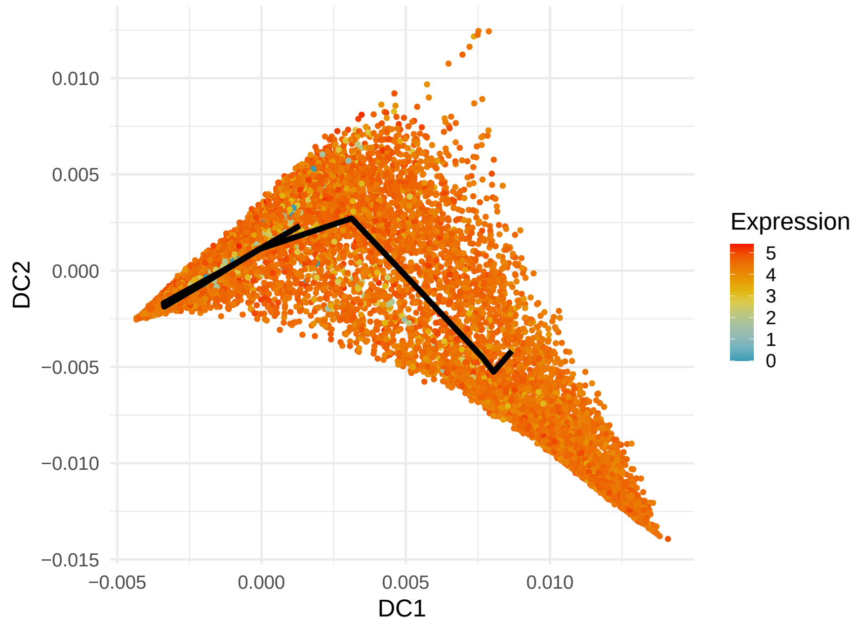
RPL41 Expression along Lineage 2 (R= 0.401)
