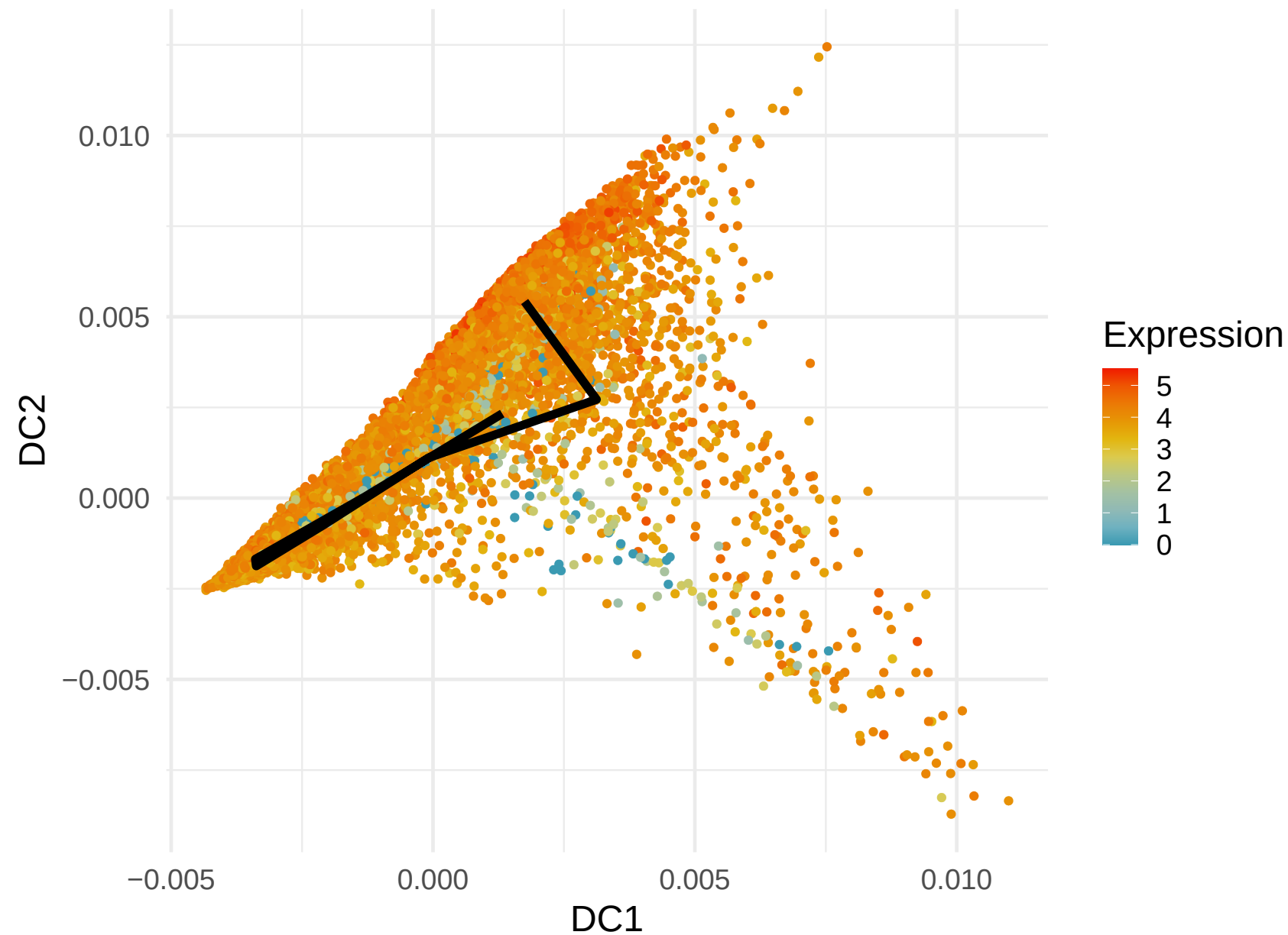
RPL39 Expression along Lineage 3 ( R = 0.544 )
