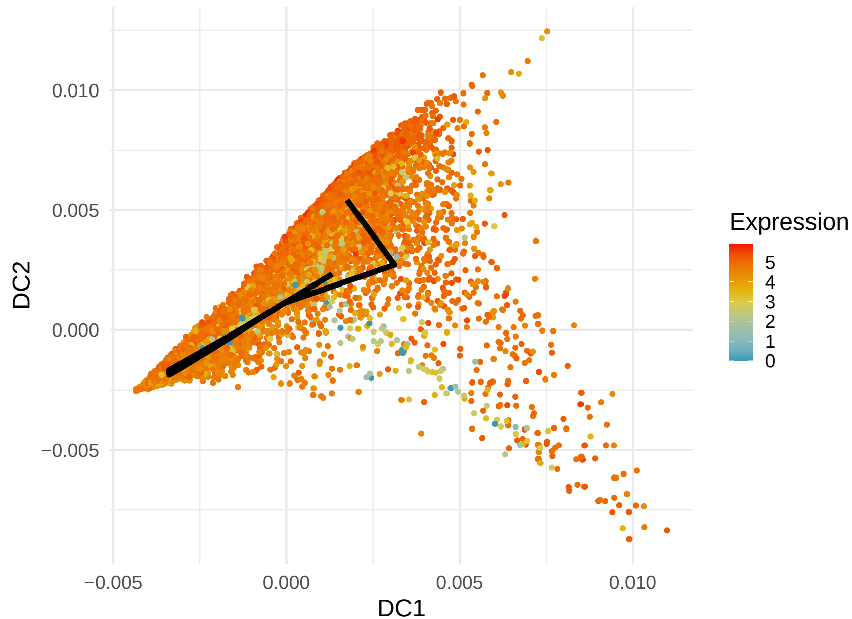
RPS27 Expression along Lineage 3 ( R = 0.566 )
