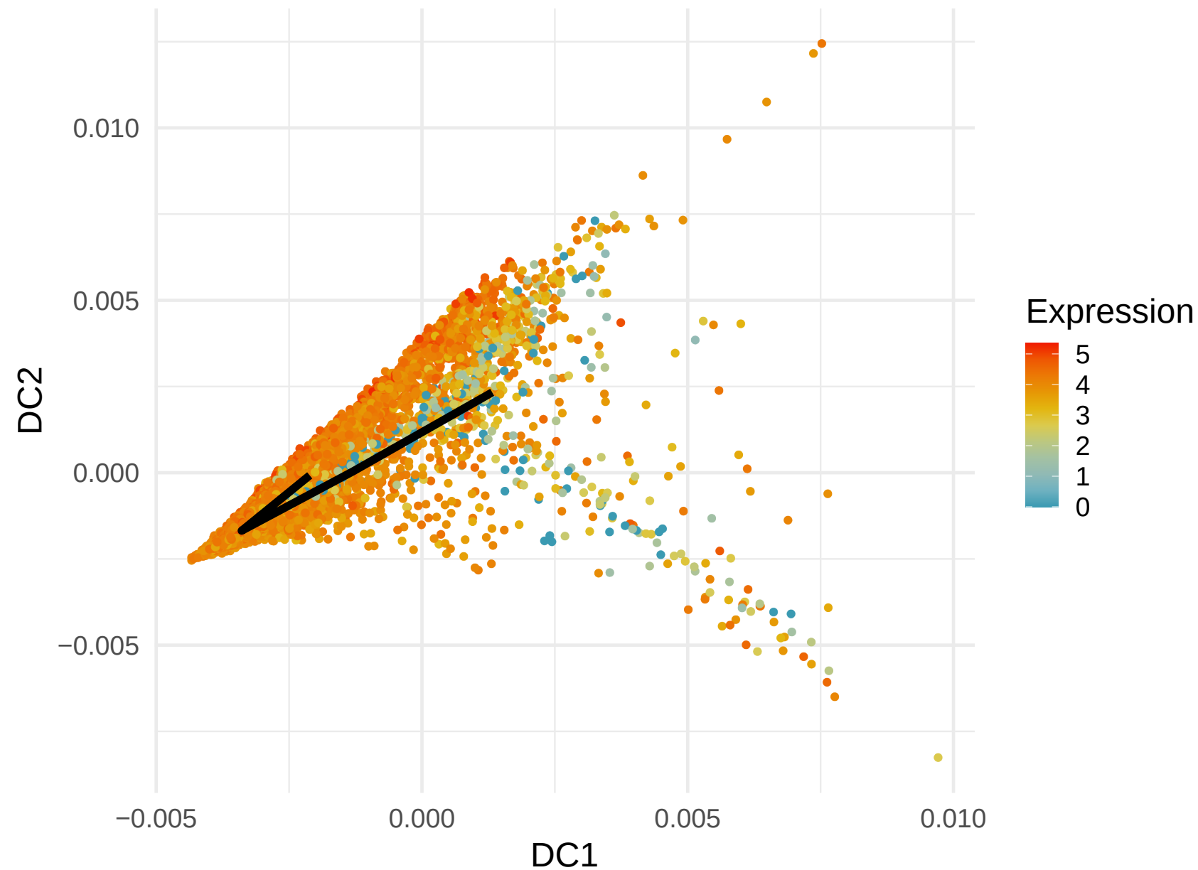
RPL39 Expression along Lineage 4 ( R = 0.579 )
