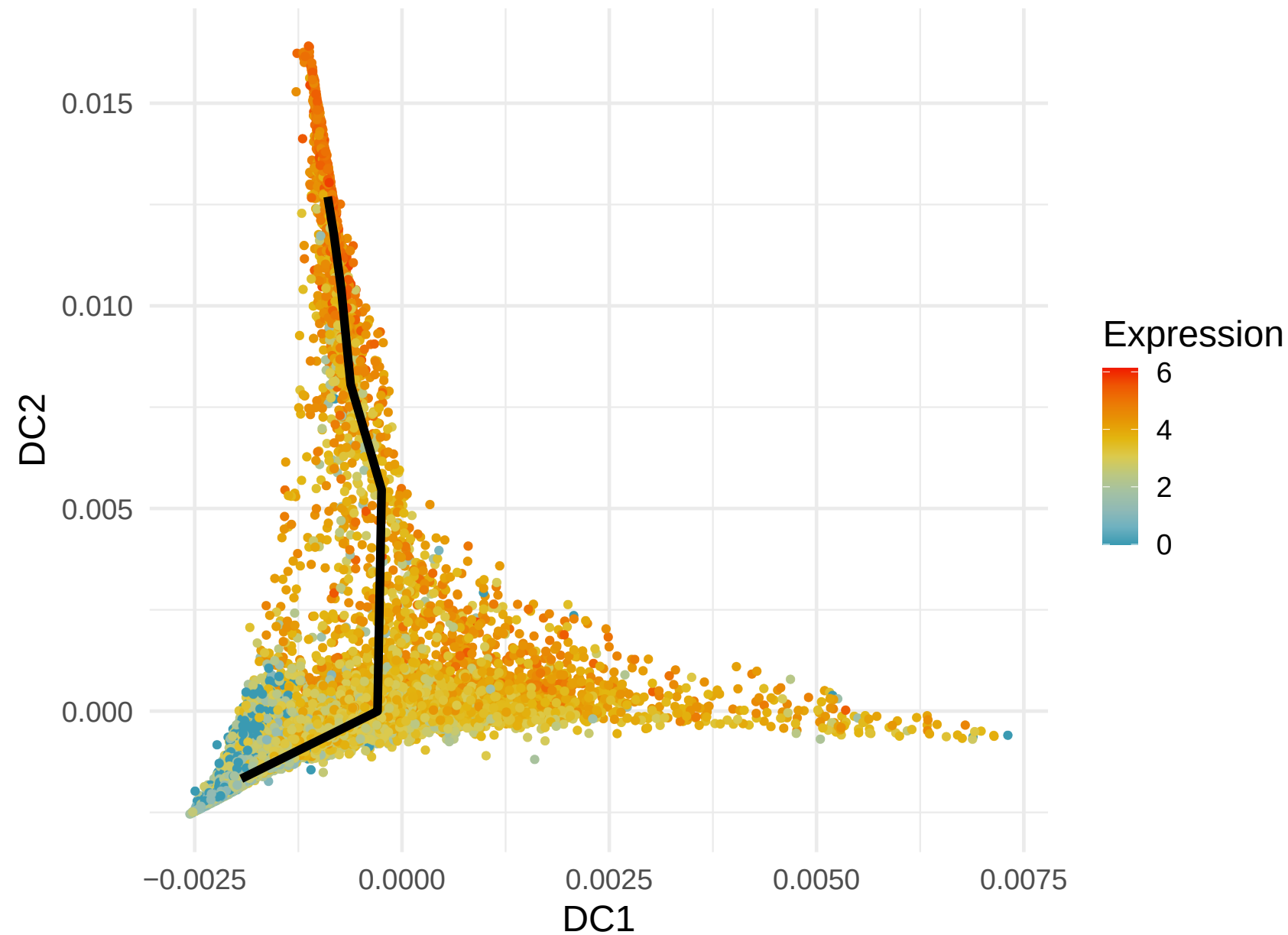
HLA-DRA Expression along Lineage 1 (R= 0.412)
