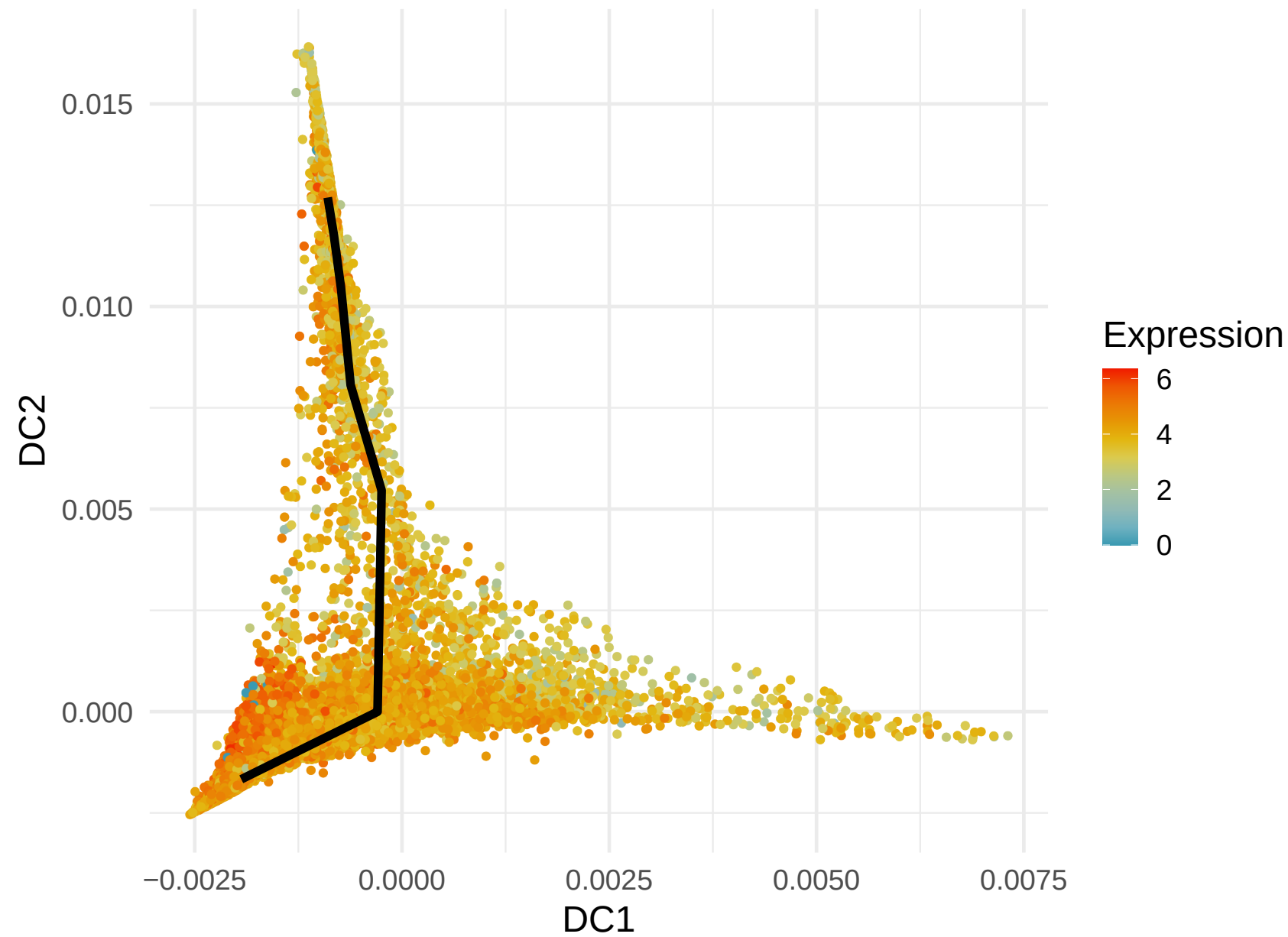
MT-CO 2 Expression along Lineage 1 ( R = -0.372 )
