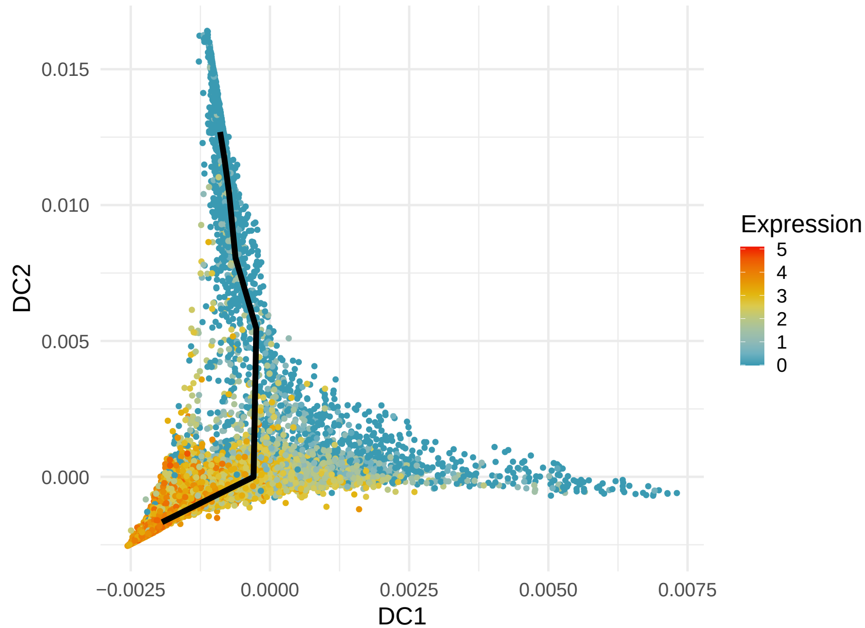
VCAN Expression along Lineage 1 ( R = -0.387 )
