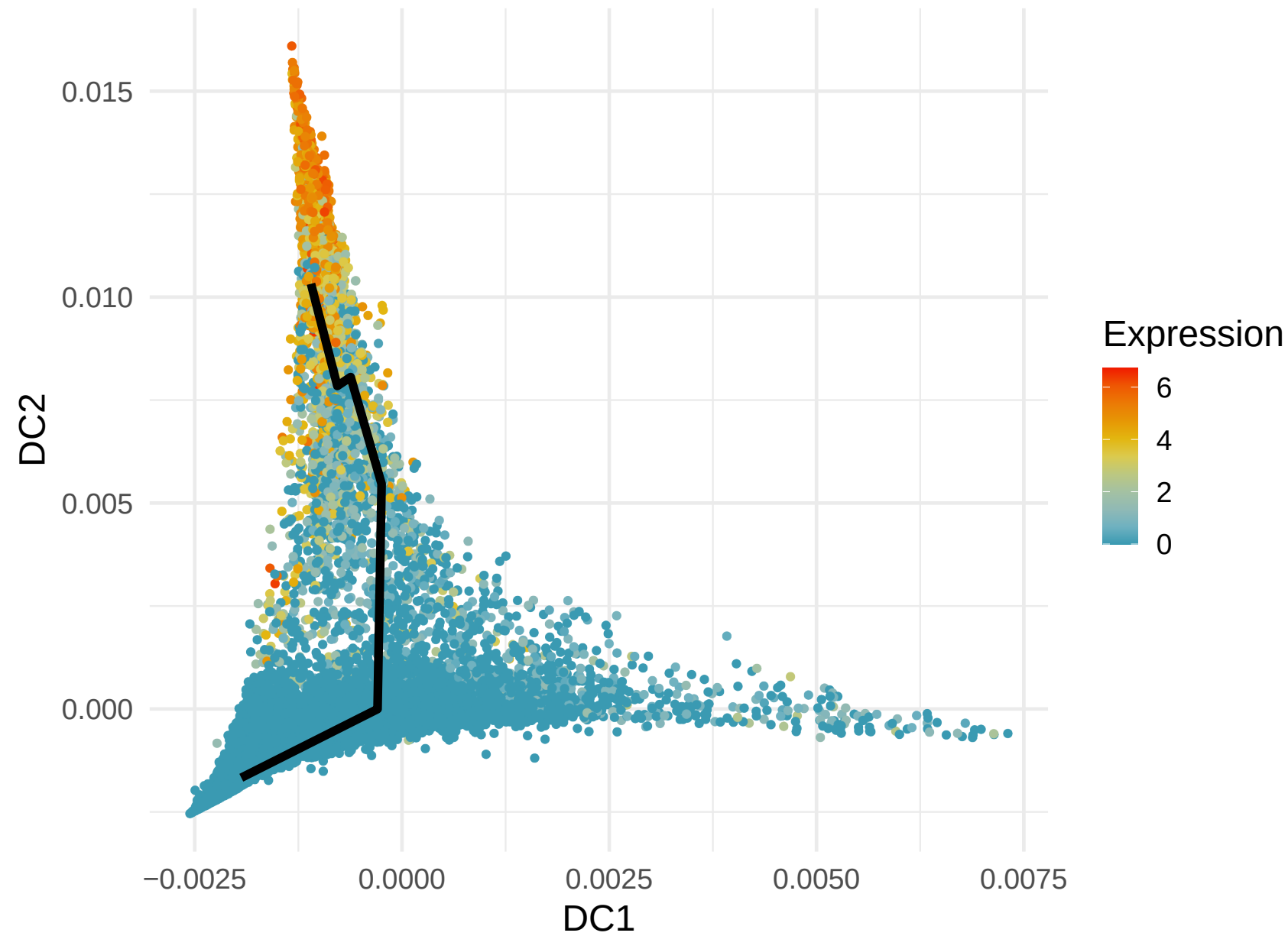
APOE Expression along Lineage 2 ( R = 0.381 )
