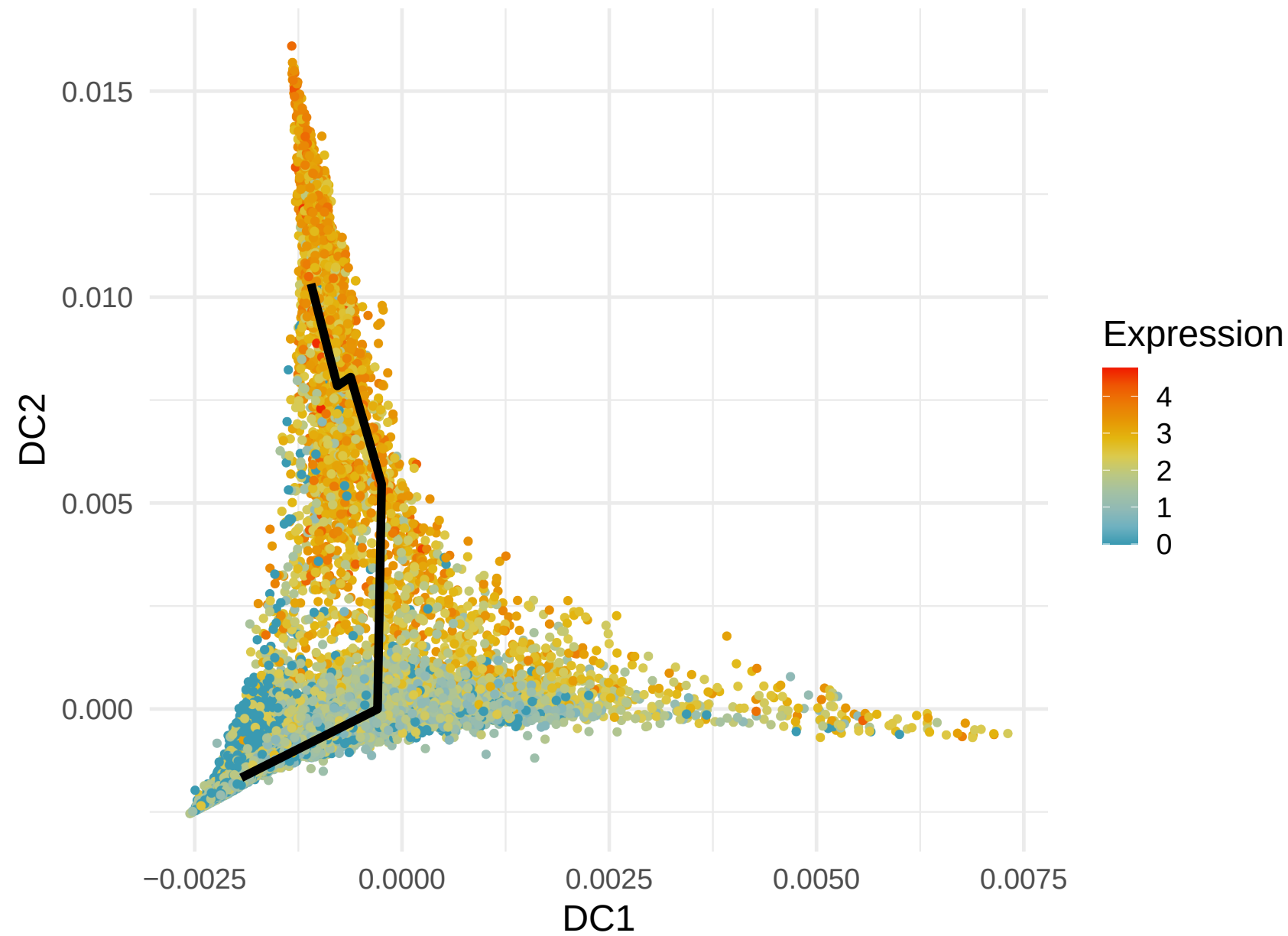
CD63 Expression along Lineage 2 ( R = 0.346 )
